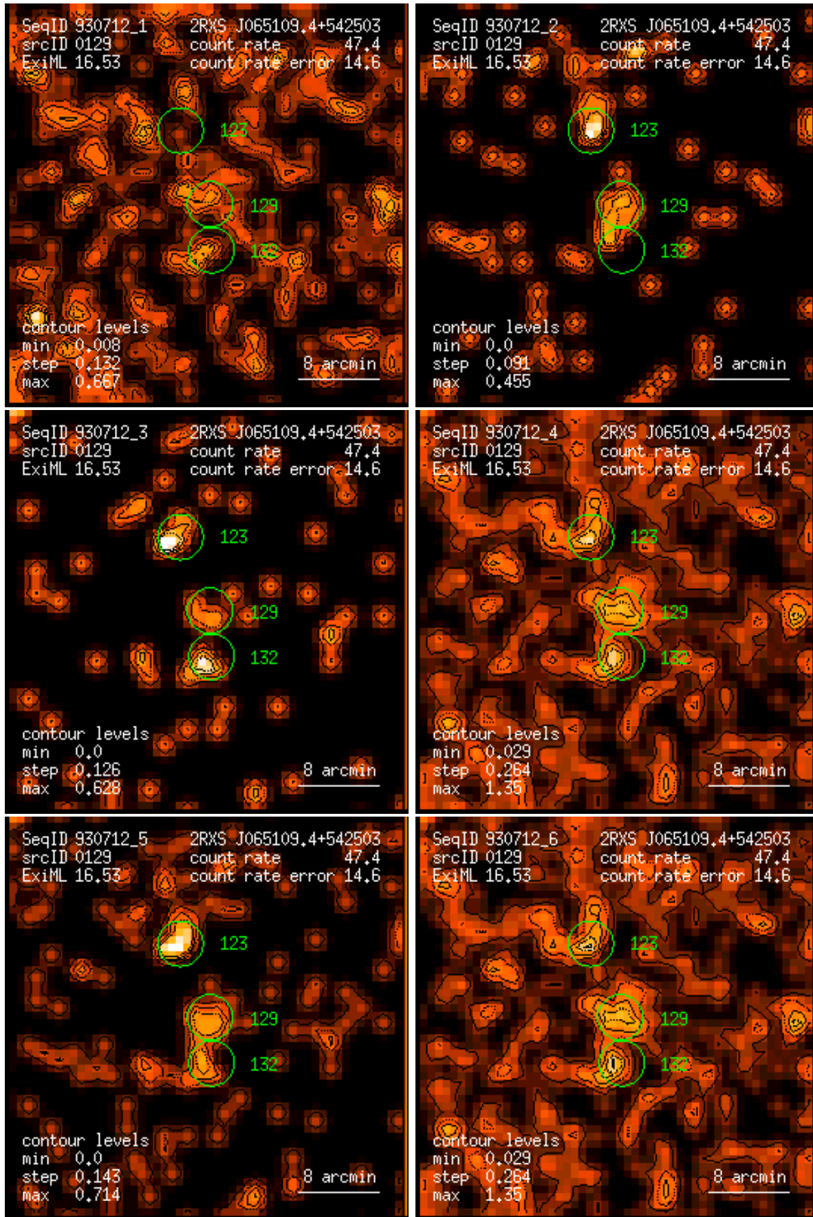
Figure 129: RASS 930712: detection 0129: band rate images, Gaussian filter: (1) PSPC channels 11 – 41, (2) 52 – 90, (3) 91 – 201, (4) 11 – 235, (5) 52 – 201, (6) 11 – 201. Broad band rates in counts/ks. Band rate contour levels in counts/ks/arcmin 2 .
