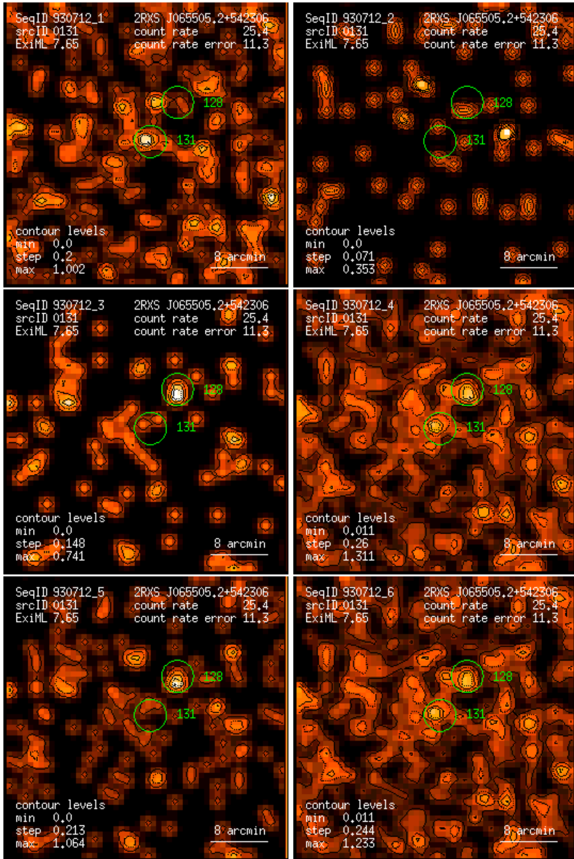
Figure 131: RASS 930712: detection 0131: band rate images, Gaussian filter: (1) PSPC channels 11 – 41, (2) 52 – 90, (3) 91 – 201, (4) 11 – 235, (5) 52 – 201, (6) 11 – 201. Broad band rates in counts/ks. Band rate contour levels in counts/ks/arcmin 2 .
