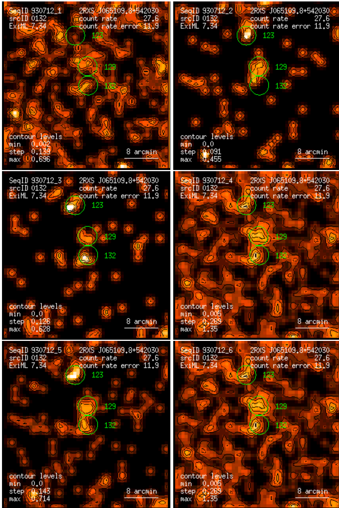
Figure 132: RASS 930712: detection 0132: band rate images, Gaussian filter: (1) PSPC channels 11 – 41, (2) 52 – 90, (3) 91 – 201, (4) 11 – 235, (5) 52 – 201, (6) 11 – 201. Broad band rates in counts/ks. Band rate contour levels in counts/ks/arcmin 2 .
