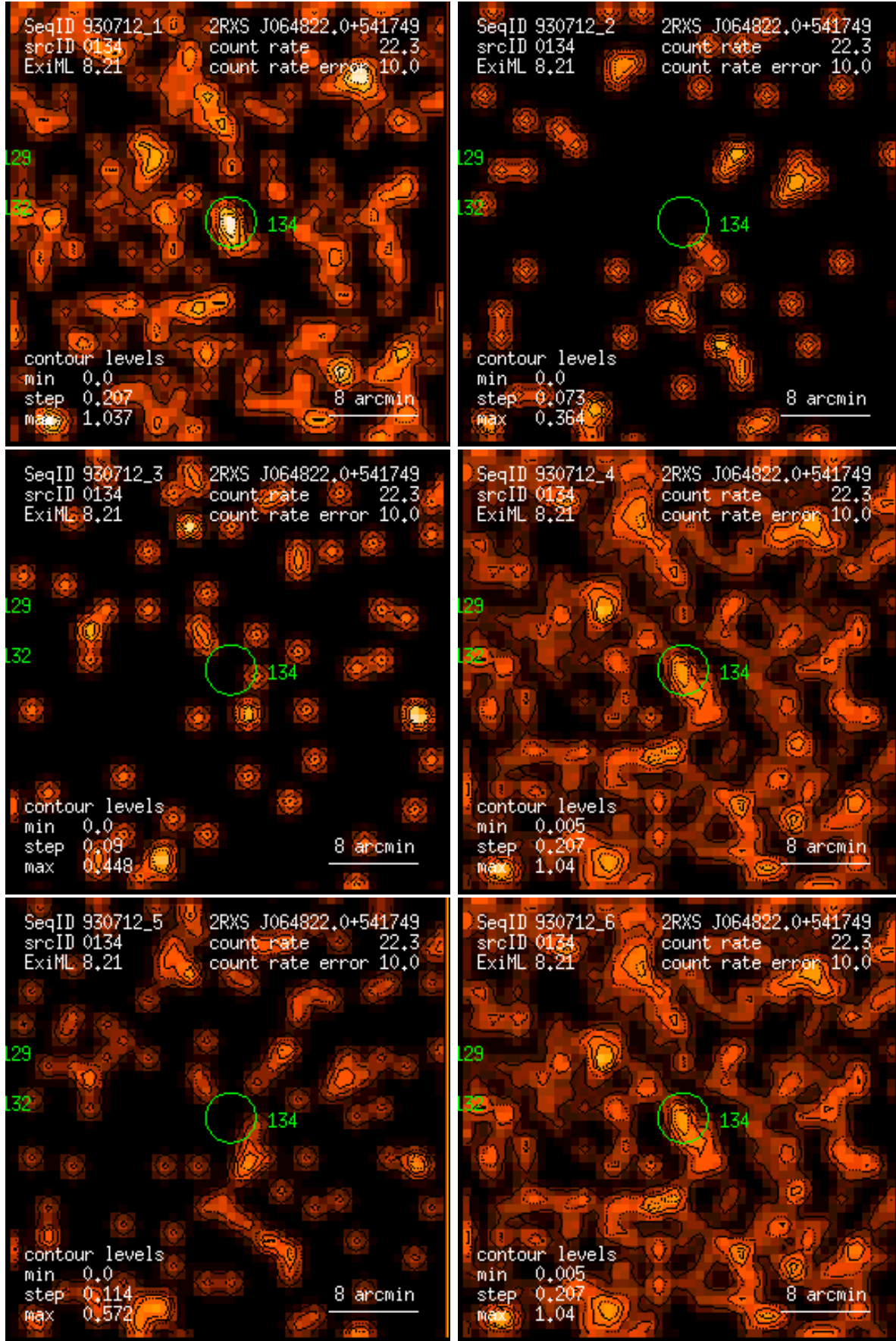
Figure 134: RASS 930712: detection 0134: band rate images, Gaussian filter: (1) PSPC channels 11 – 41, (2) 52 – 90, (3) 91 – 201, (4) 11 – 235, (5) 52 – 201, (6) 11 – 201. Broad band rates in counts/ks. Band rate contour levels in counts/ks/arcmin 2 .
