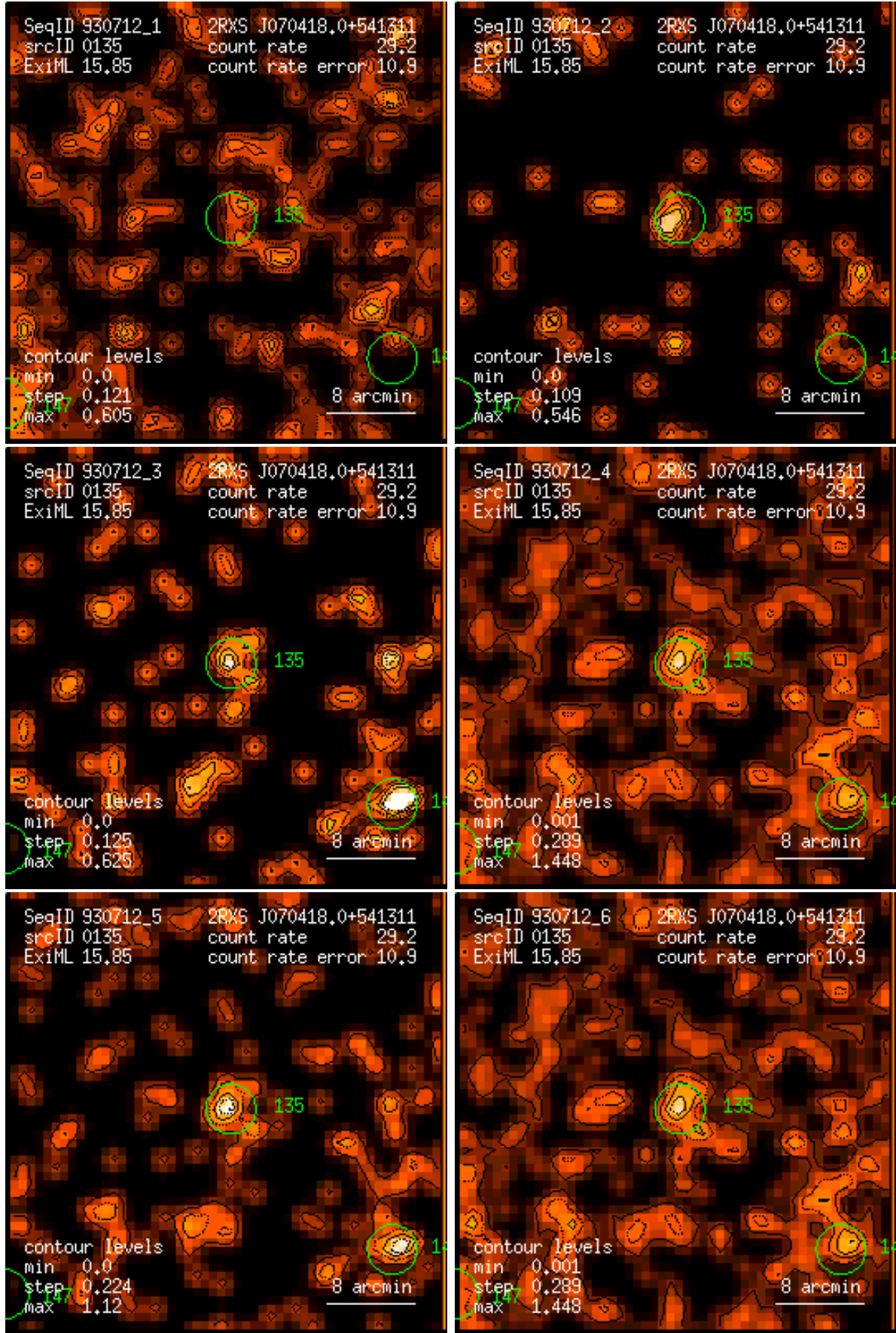
Figure 135: RASS 930712: detection 0135: band rate images, Gaussian filter: (1) PSPC channels 11 – 41, (2) 52 – 90, (3) 91 – 201, (4) 11 – 235, (5) 52 – 201, (6) 11 – 201. Broad band rates in counts/ks. Band rate contour levels in counts/ks/arcmin 2 .
