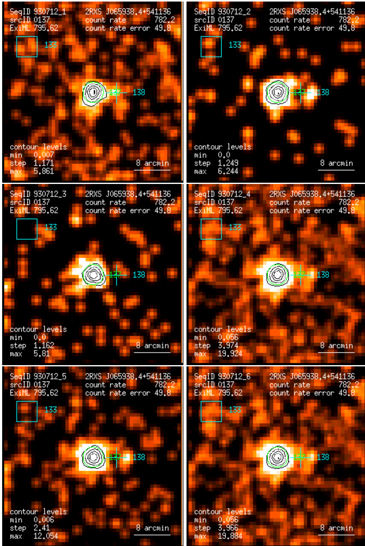
Figure 137: RASS 930712: detection 0137: band rate images, Gaussian filter: (1) PSPC channels 11 – 41, (2) 52 – 90, (3) 91 – 201, (4) 11 – 235, (5) 52 – 201, (6) 11 – 201. Broad band rates in counts/ks. Band rate contour levels in counts/ks/arcmin 2 .
