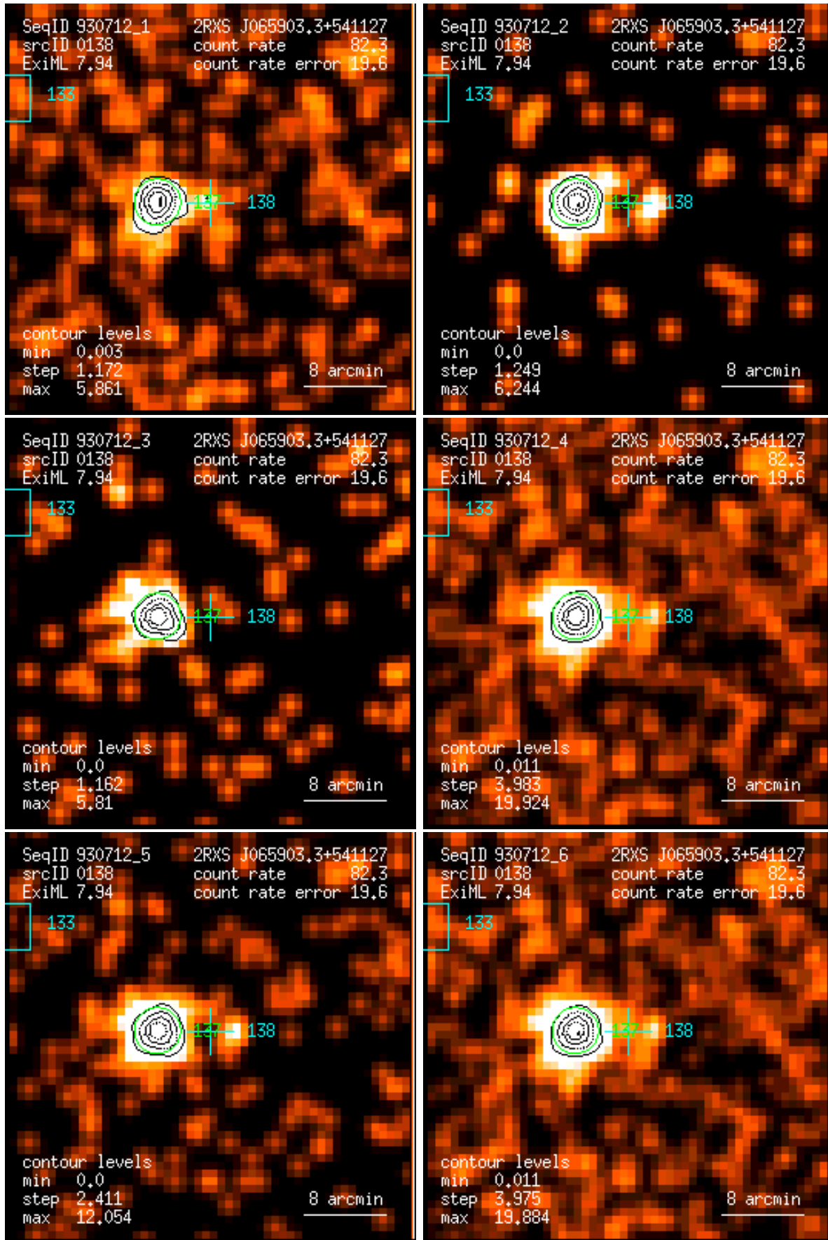
Figure 138: RASS 930712: detection 0138: band rate images, Gaussian filter: (1) PSPC channels 11 – 41, (2) 52 – 90, (3) 91 – 201, (4) 11 – 235, (5) 52 – 201, (6) 11 – 201. Broad band rates in counts/ks. Band rate contour levels in counts/ks/arcmin 2 .
