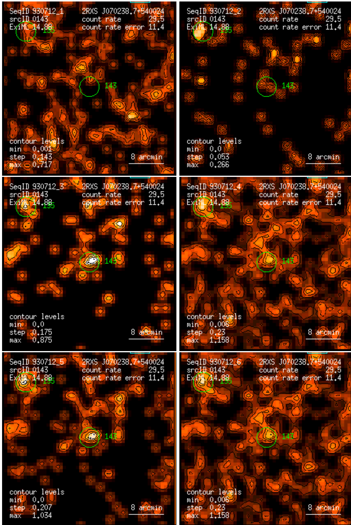
Figure 143: RASS 930712: detection 0143: band rate images, Gaussian filter: (1) PSPC channels 11 – 41, (2) 52 – 90, (3) 91 – 201, (4) 11 – 235, (5) 52 – 201, (6) 11 – 201. Broad band rates in counts/ks. Band rate contour levels in counts/ks/arcmin 2 .
