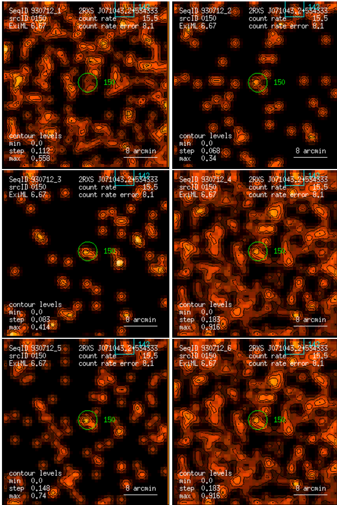
Figure 150: RASS 930712: detection 0150: band rate images, Gaussian filter: (1) PSPC channels 11 – 41, (2) 52 – 90, (3) 91 – 201, (4) 11 – 235, (5) 52 – 201, (6) 11 – 201. Broad band rates in counts/ks. Band rate contour levels in counts/ks/arcmin 2 .
