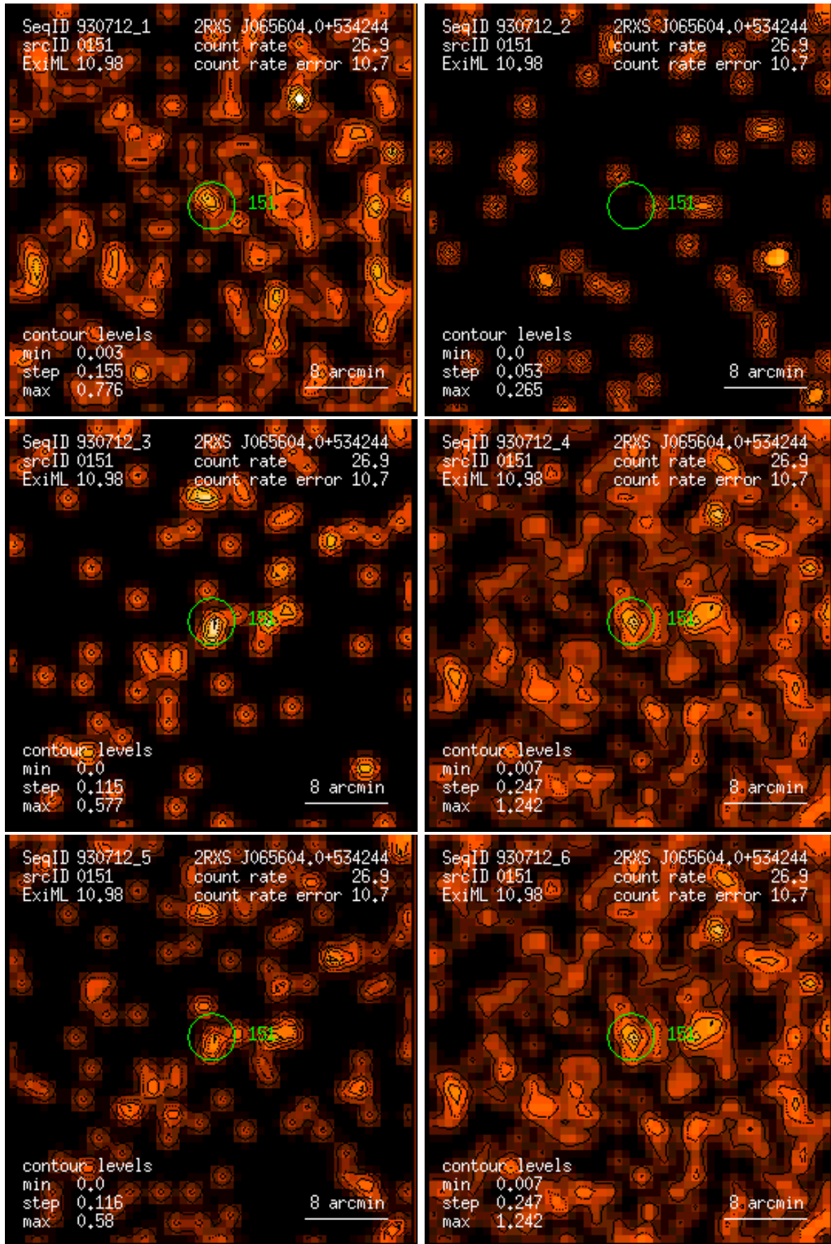
Figure 151: RASS 930712: detection 0151: band rate images, Gaussian filter: (1) PSPC channels 11 – 41, (2) 52 – 90, (3) 91 – 201, (4) 11 – 235, (5) 52 – 201, (6) 11 – 201. Broad band rates in counts/ks. Band rate contour levels in counts/ks/arcmin 2 .
