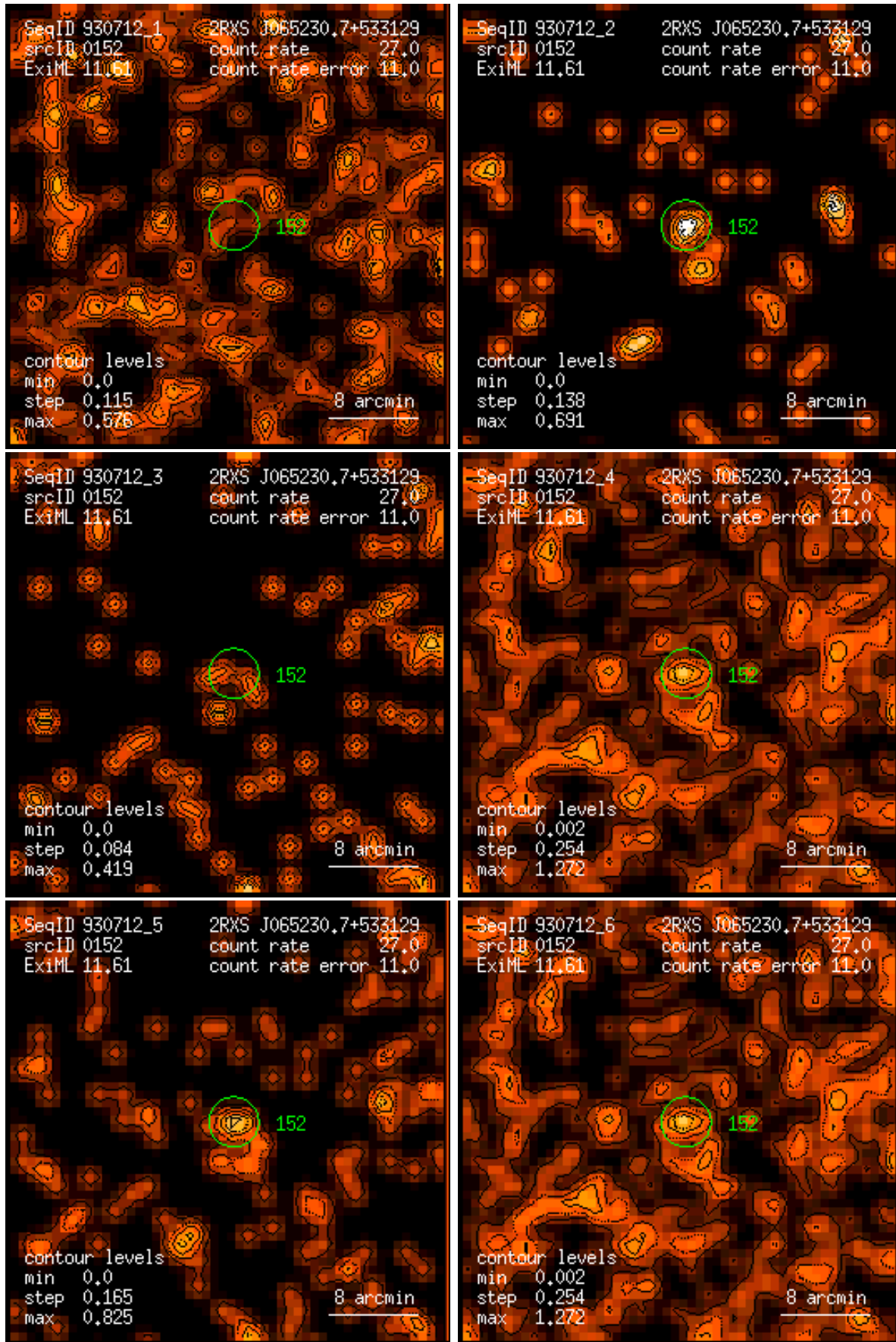
Figure 152: RASS 930712: detection 0152: band rate images, Gaussian filter: (1) PSPC channels 11 – 41, (2) 52 – 90, (3) 91 – 201, (4) 11 – 235, (5) 52 – 201, (6) 11 – 201. Broad band rates in counts/ks. Band rate contour levels in counts/ks/arcmin 2 .
