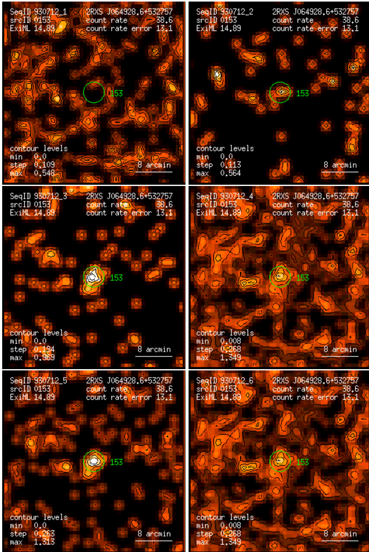
Figure 153: RASS 930712: detection 0153: band rate images, Gaussian filter: (1) PSPC channels 11 – 41, (2) 52 – 90, (3) 91 – 201, (4) 11 – 235, (5) 52 – 201, (6) 11 – 201. Broad band rates in counts/ks. Band rate contour levels in counts/ks/arcmin 2 .
