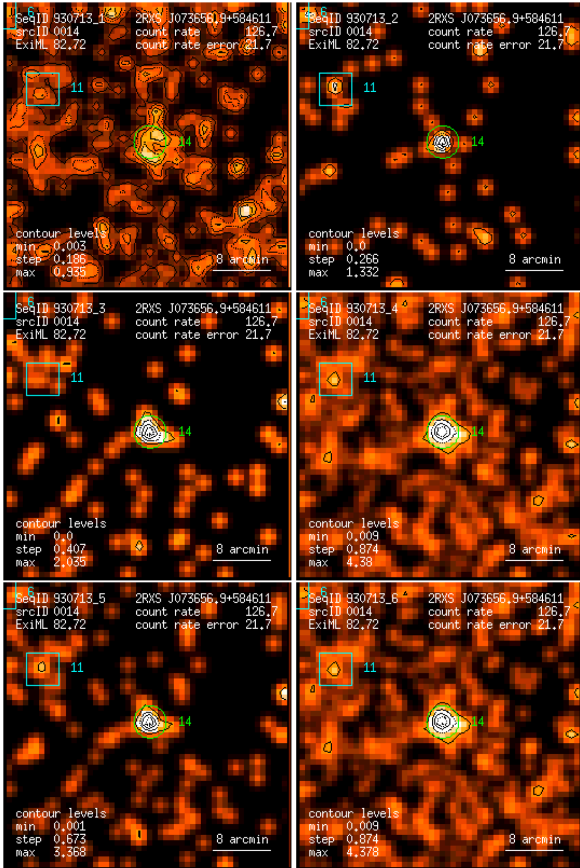
Figure 14: RASS 930713: detection 0014: band rate images, Gaussian filter: (1) PSPC channels 11 – 41, (2) 52 – 90, (3) 91 – 201, (4) 11 – 235, (5) 52 – 201, (6) 11 – 201. Broad band rates in counts/ks. Band rate contour levels in counts/ks/arcmin 2 .
