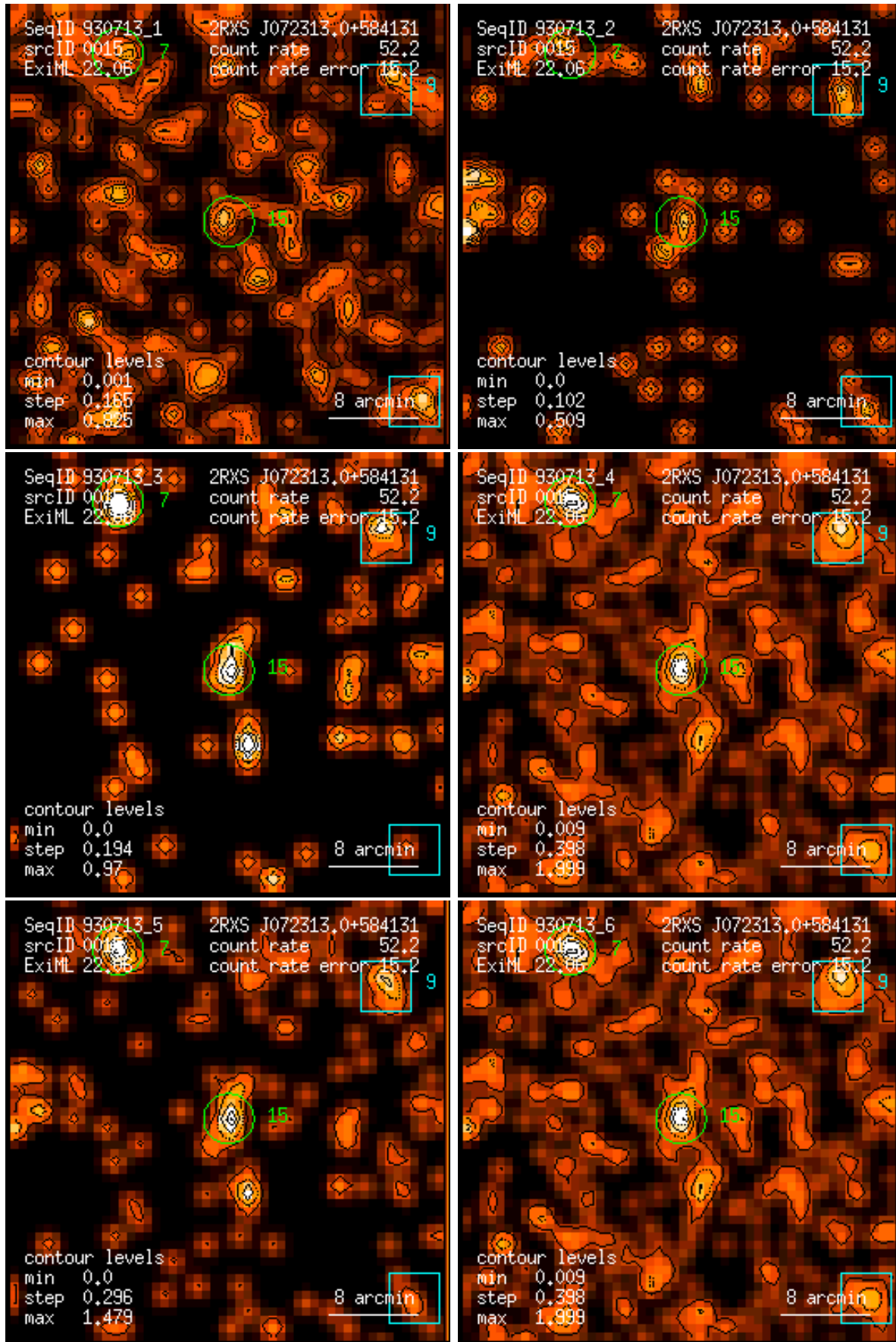
Figure 15: RASS 930713: detection 0015: band rate images, Gaussian filter: (1) PSPC channels 11 – 41, (2) 52 – 90, (3) 91 – 201, (4) 11 – 235, (5) 52 – 201, (6) 11 – 201. Broad band rates in counts/ks. Band rate contour levels in counts/ks/arcmin 2 .
