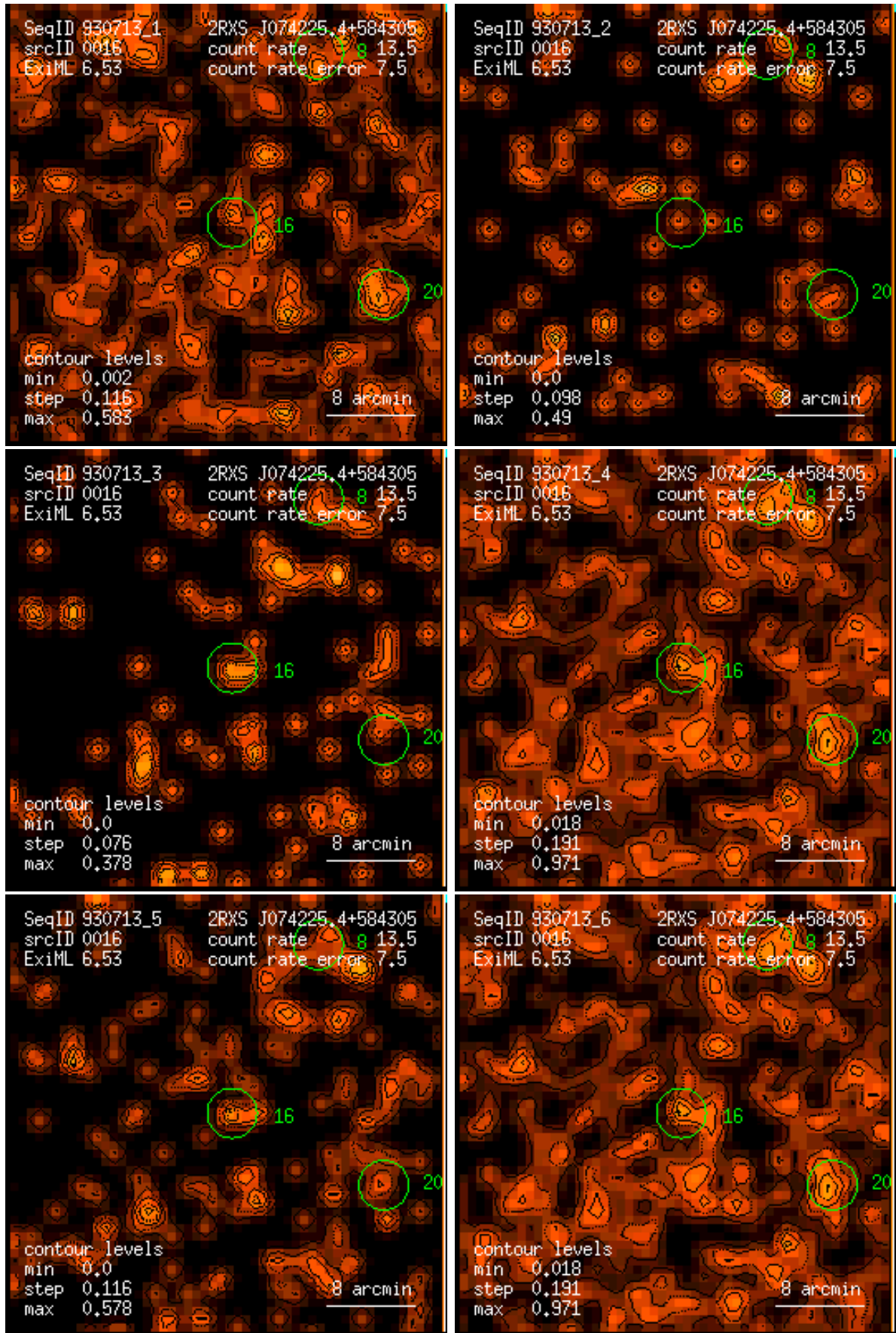
Figure 16: RASS 930713: detection 0016: band rate images, Gaussian filter: (1) PSPC channels 11 – 41, (2) 52 – 90, (3) 91 – 201, (4) 11 – 235, (5) 52 – 201, (6) 11 – 201. Broad band rates in counts/ks. Band rate contour levels in counts/ks/arcmin 2 .
