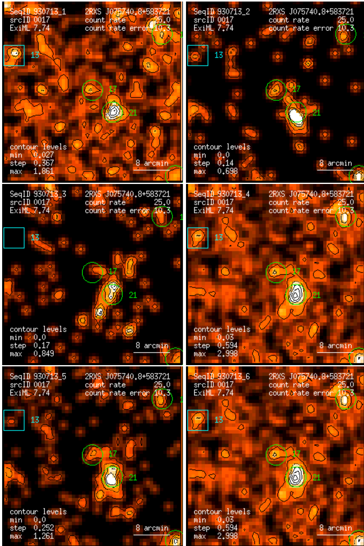
Figure 17: RASS 930713: detection 0017: band rate images, Gaussian filter: (1) PSPC channels 11 – 41, (2) 52 – 90, (3) 91 – 201, (4) 11 – 235, (5) 52 – 201, (6) 11 – 201. Broad band rates in counts/ks. Band rate contour levels in counts/ks/arcmin 2 .
