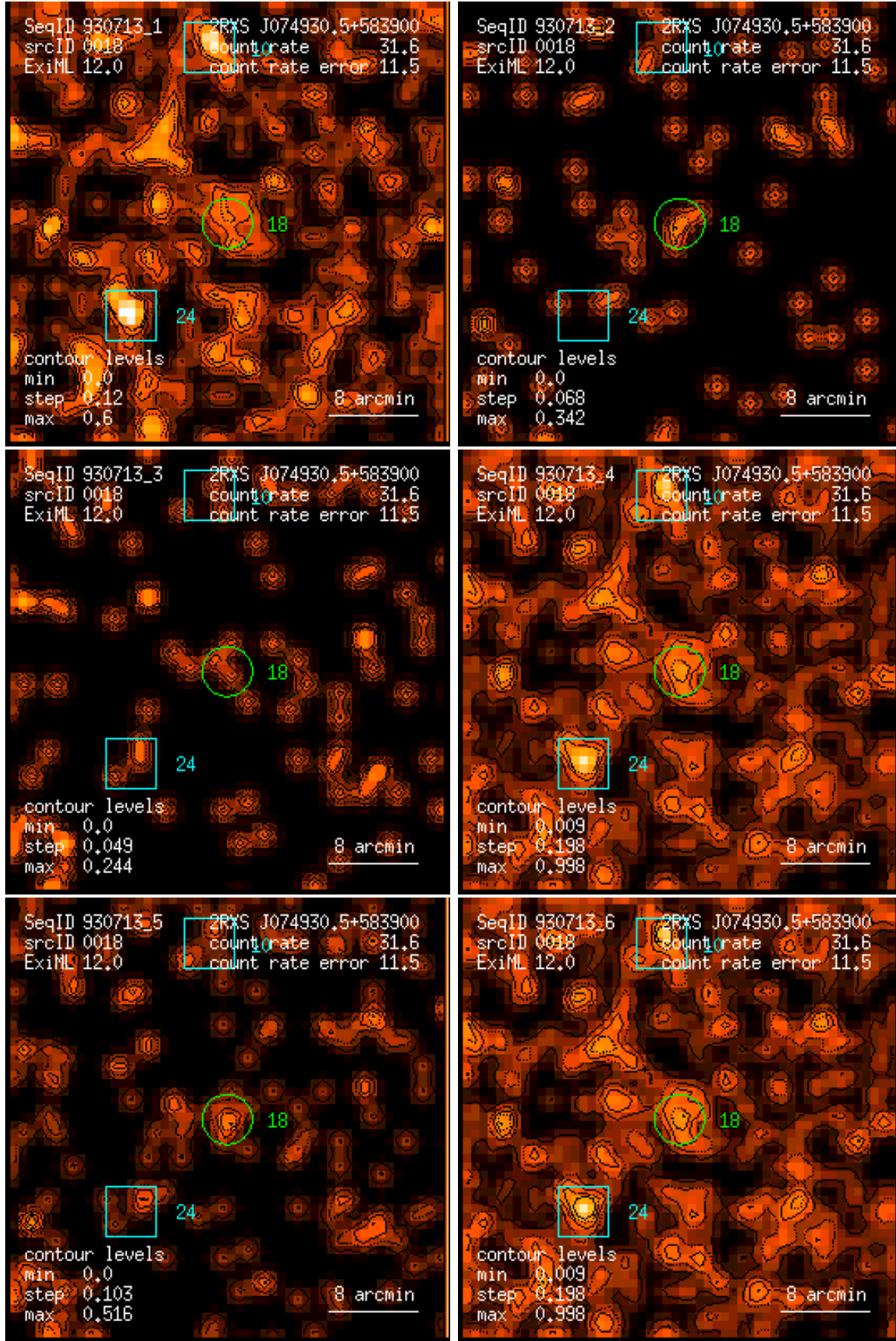
Figure 18: RASS 930713: detection 0018: band rate images, Gaussian filter: (1) PSPC channels 11 – 41, (2) 52 – 90, (3) 91 – 201, (4) 11 – 235, (5) 52 – 201, (6) 11 – 201. Broad band rates in counts/ks. Band rate contour levels in counts/ks/arcmin 2 .
