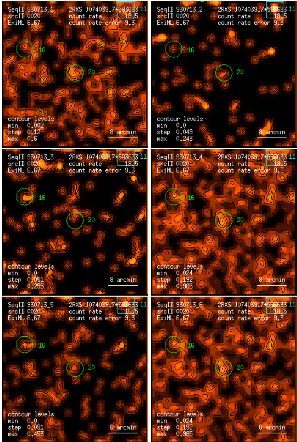
Figure 20: RASS 930713: detection 0020: band rate images, Gaussian filter: (1) PSPC channels 11 – 41, (2) 52 – 90, (3) 91 – 201, (4) 11 – 235, (5) 52 – 201, (6) 11 – 201. Broad band rates in counts/ks. Band rate contour levels in counts/ks/arcmin 2 .
