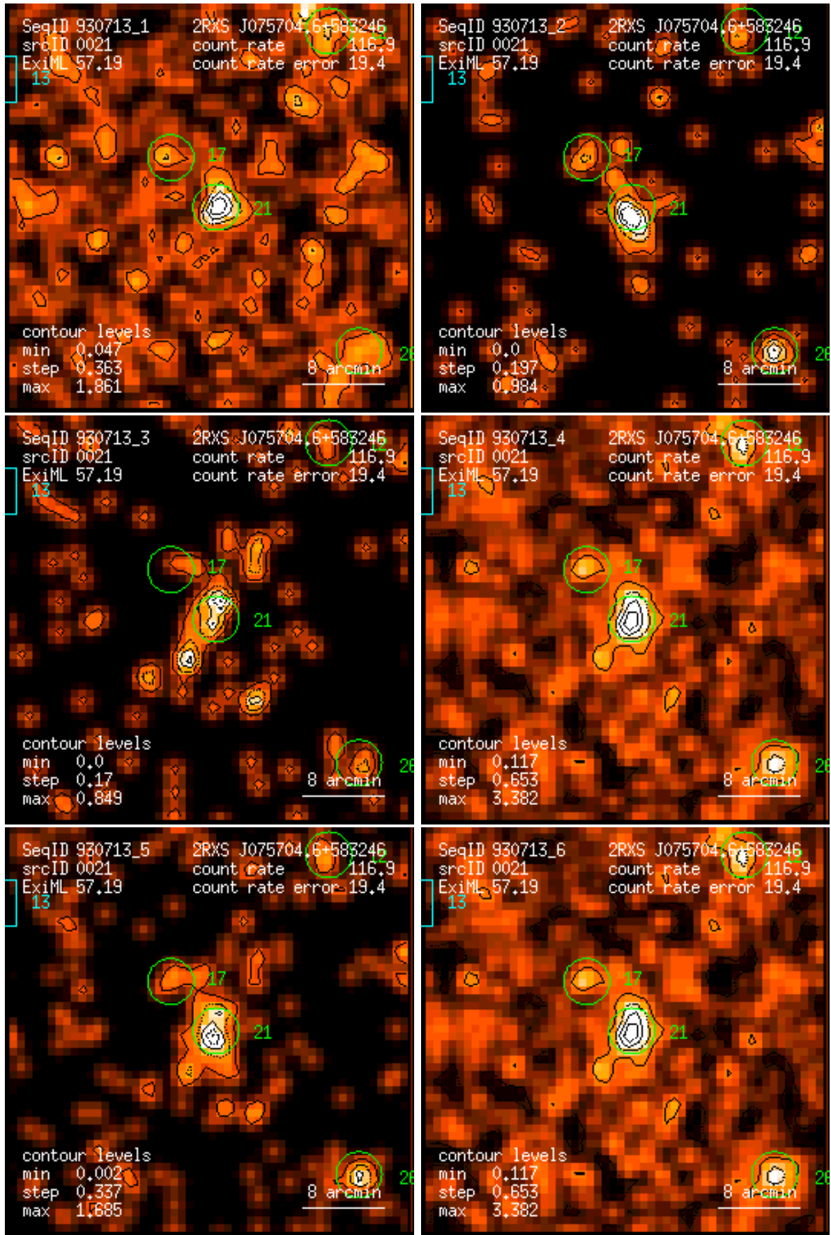
Figure 21: RASS 930713: detection 0021: band rate images, Gaussian filter: (1) PSPC channels 11 – 41, (2) 52 – 90, (3) 91 – 201, (4) 11 – 235, (5) 52 – 201, (6) 11 – 201. Broad band rates in counts/ks. Band rate contour levels in counts/ks/arcmin 2 .
