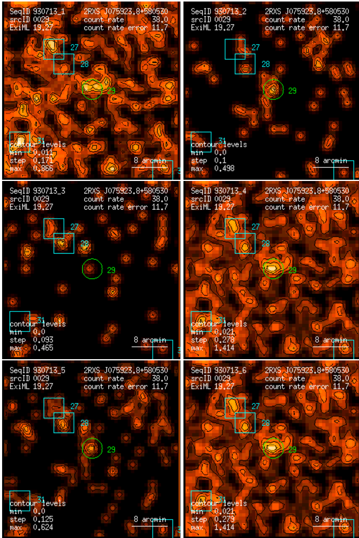
Figure 29: RASS 930713: detection 0029: band rate images, Gaussian filter: (1) PSPC channels 11 – 41, (2) 52 – 90, (3) 91 – 201, (4) 11 – 235, (5) 52 – 201, (6) 11 – 201. Broad band rates in counts/ks. Band rate contour levels in counts/ks/arcmin 2 .
