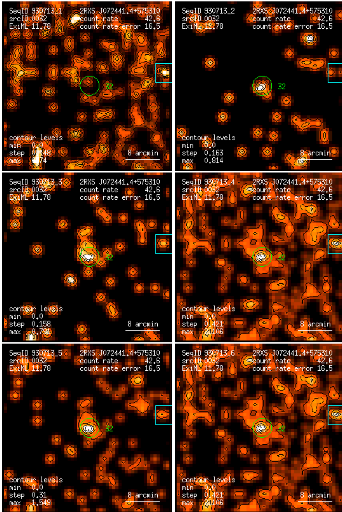
Figure 32: RASS 930713: detection 0032: band rate images, Gaussian filter: (1) PSPC channels 11 – 41, (2) 52 – 90, (3) 91 – 201, (4) 11 – 235, (5) 52 – 201, (6) 11 – 201. Broad band rates in counts/ks. Band rate contour levels in counts/ks/arcmin 2 .
