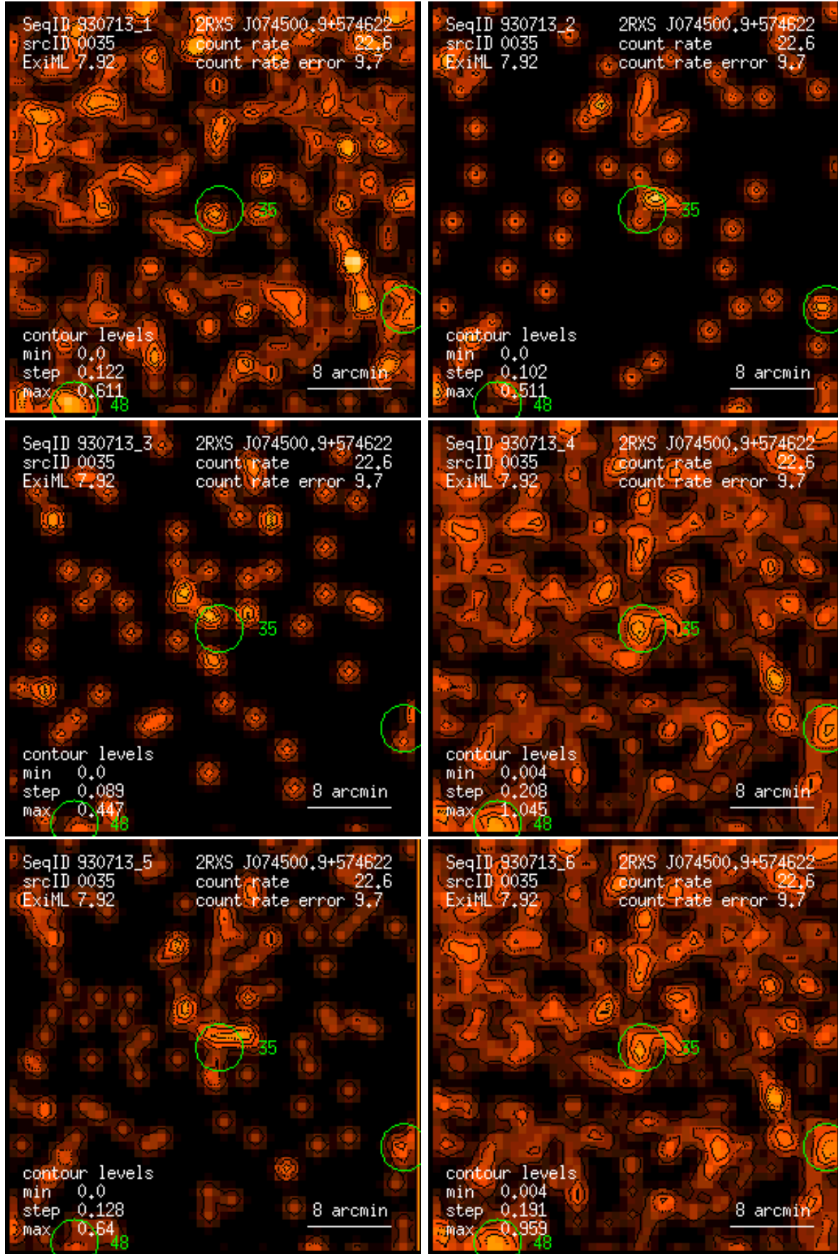
Figure 35: RASS 930713: detection 0035: band rate images, Gaussian filter: (1) PSPC channels 11 – 41, (2) 52 – 90, (3) 91 – 201, (4) 11 – 235, (5) 52 – 201, (6) 11 – 201. Broad band rates in counts/ks. Band rate contour levels in counts/ks/arcmin 2 .
