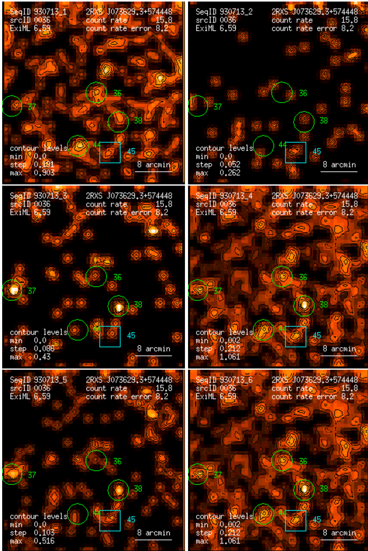
Figure 36: RASS 930713: detection 0036: band rate images, Gaussian filter: (1) PSPC channels 11 – 41, (2) 52 – 90, (3) 91 – 201, (4) 11 – 235, (5) 52 – 201, (6) 11 – 201. Broad band rates in counts/ks. Band rate contour levels in counts/ks/arcmin 2 .
