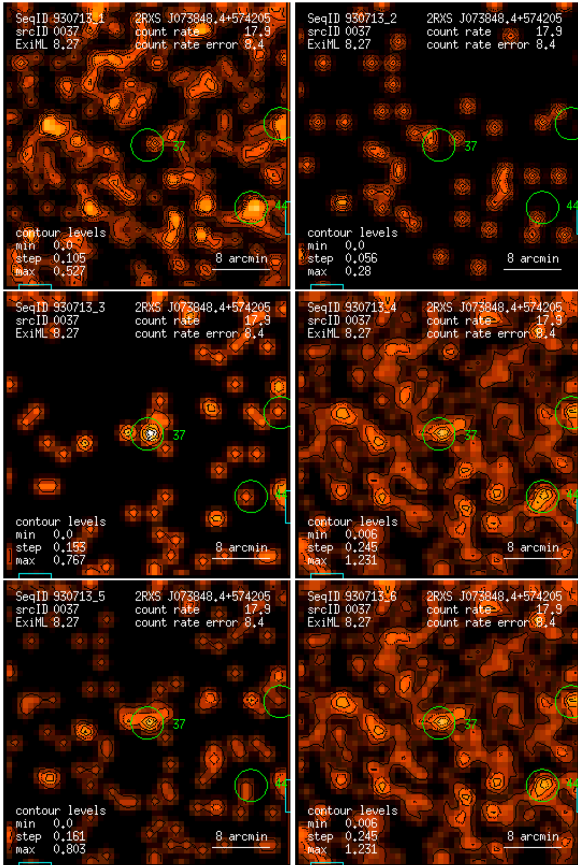
Figure 37: RASS 930713: detection 0037: band rate images, Gaussian filter: (1) PSPC channels 11 – 41, (2) 52 – 90, (3) 91 – 201, (4) 11 – 235, (5) 52 – 201, (6) 11 – 201. Broad band rates in counts/ks. Band rate contour levels in counts/ks/arcmin 2 .
