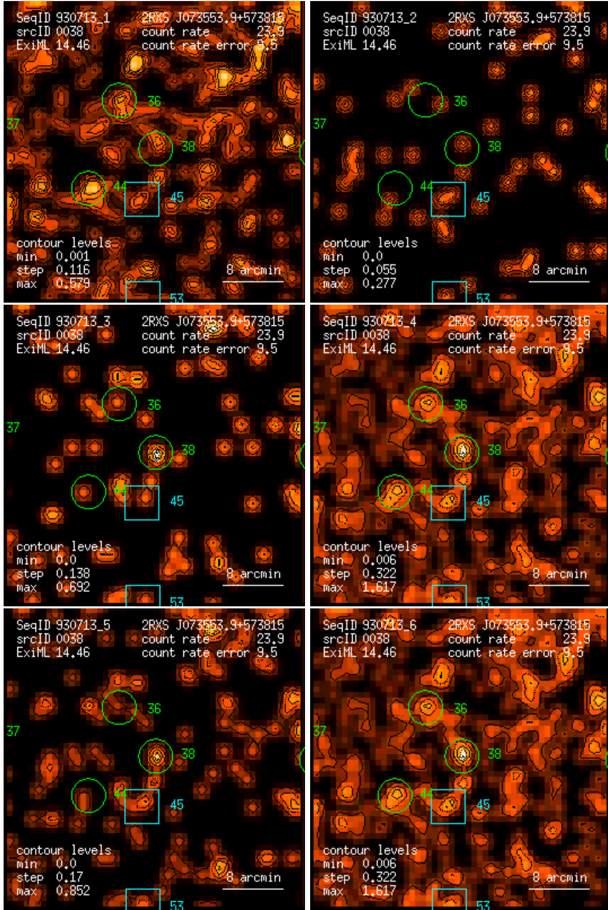
Figure 38: RASS 930713: detection 0038: band rate images, Gaussian filter: (1) PSPC channels 11 – 41, (2) 52 – 90, (3) 91 – 201, (4) 11 – 235, (5) 52 – 201, (6) 11 – 201. Broad band rates in counts/ks. Band rate contour levels in counts/ks/arcmin 2 .
