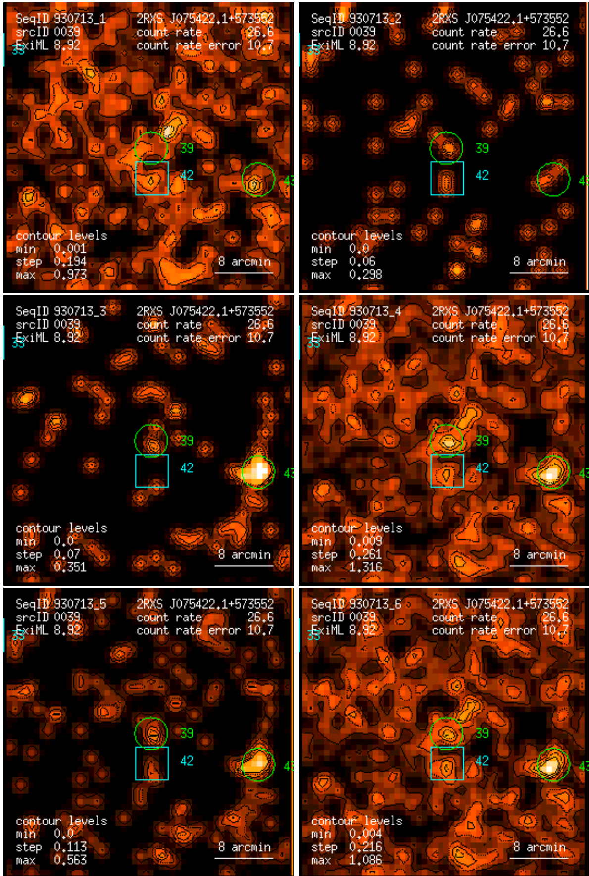
Figure 39: RASS 930713: detection 0039: band rate images, Gaussian filter: (1) PSPC channels 11 – 41, (2) 52 – 90, (3) 91 – 201, (4) 11 – 235, (5) 52 – 201, (6) 11 – 201. Broad band rates in counts/ks. Band rate contour levels in counts/ks/arcmin 2 .
