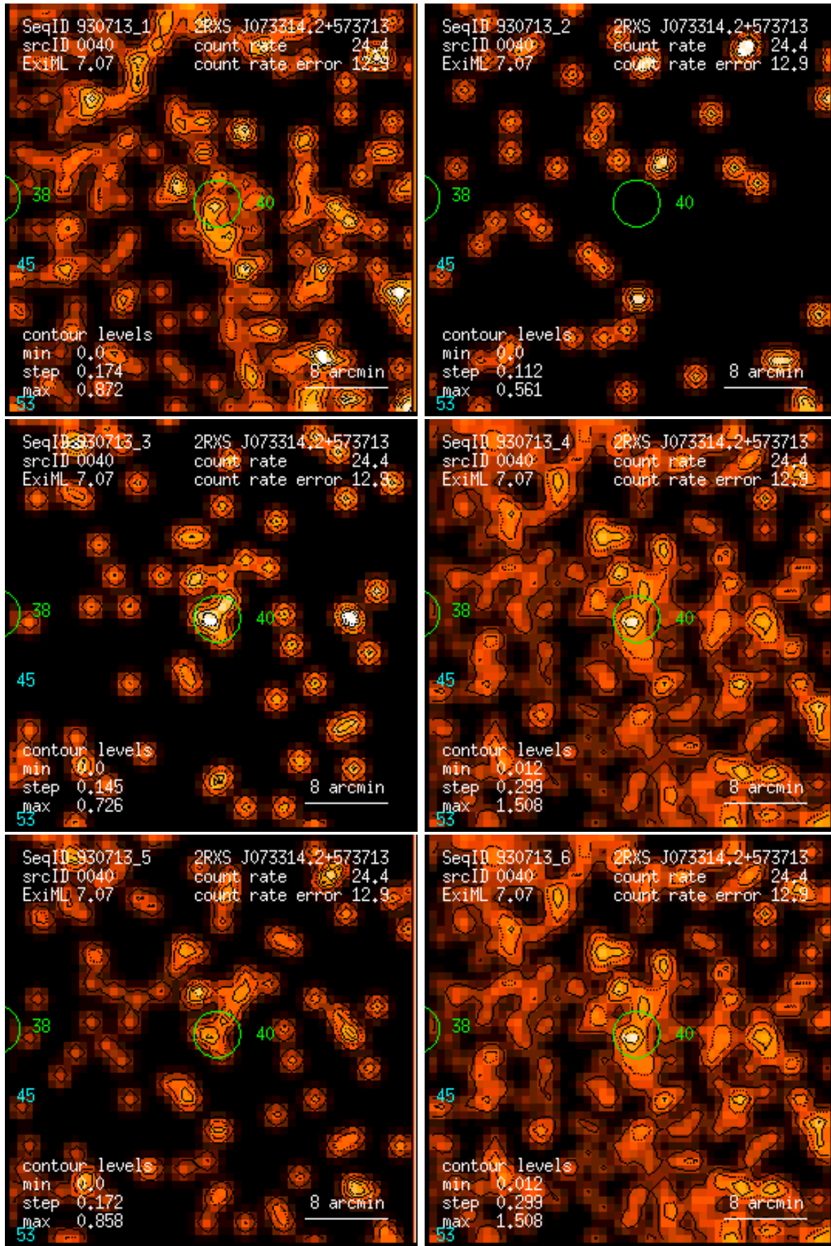
Figure 40: RASS 930713: detection 0040: band rate images, Gaussian filter: (1) PSPC channels 11 – 41, (2) 52 – 90, (3) 91 – 201, (4) 11 – 235, (5) 52 – 201, (6) 11 – 201. Broad band rates in counts/ks. Band rate contour levels in counts/ks/arcmin 2 .
