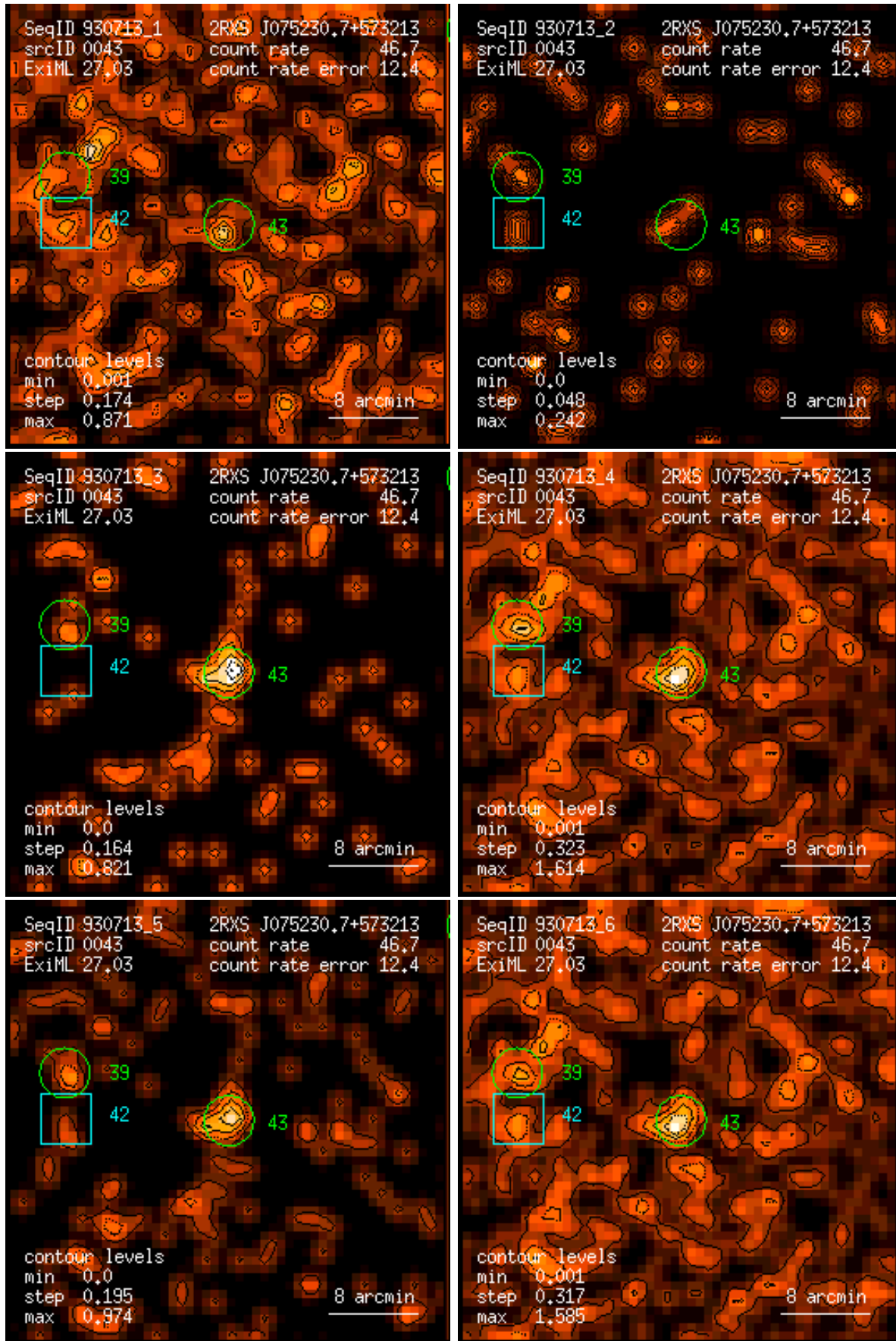
Figure 43: RASS 930713: detection 0043: band rate images, Gaussian filter: (1) PSPC channels 11 – 41, (2) 52 – 90, (3) 91 – 201, (4) 11 – 235, (5) 52 – 201, (6) 11 – 201. Broad band rates in counts/ks. Band rate contour levels in counts/ks/arcmin 2 .
