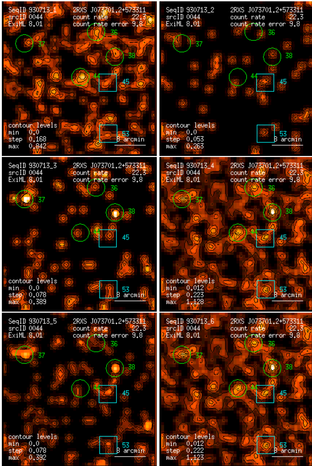
Figure 44: RASS 930713: detection 0044: band rate images, Gaussian filter: (1) PSPC channels 11 – 41, (2) 52 – 90, (3) 91 – 201, (4) 11 – 235, (5) 52 – 201, (6) 11 – 201. Broad band rates in counts/ks. Band rate contour levels in counts/ks/arcmin 2 .
