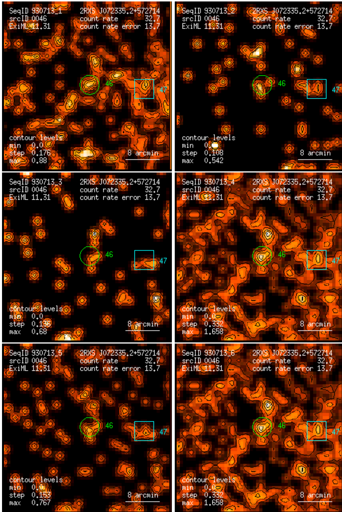
Figure 46: RASS 930713: detection 0046: band rate images, Gaussian filter: (1) PSPC channels 11 – 41, (2) 52 – 90, (3) 91 – 201, (4) 11 – 235, (5) 52 – 201, (6) 11 – 201. Broad band rates in counts/ks. Band rate contour levels in counts/ks/arcmin 2 .
