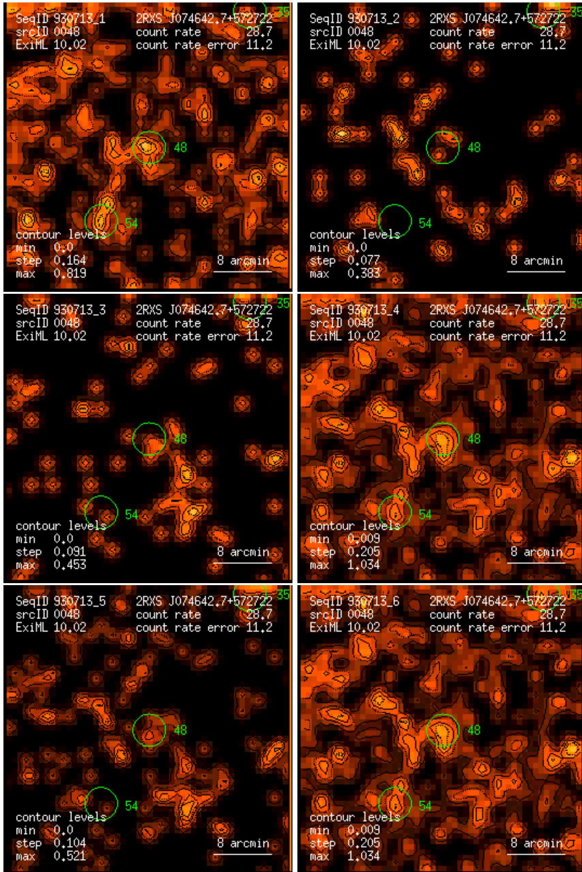
Figure 48: RASS 930713: detection 0048: band rate images, Gaussian filter: (1) PSPC channels 11 – 41, (2) 52 – 90, (3) 91 – 201, (4) 11 – 235, (5) 52 – 201, (6) 11 – 201. Broad band rates in counts/ks. Band rate contour levels in counts/ks/arcmin 2 .
