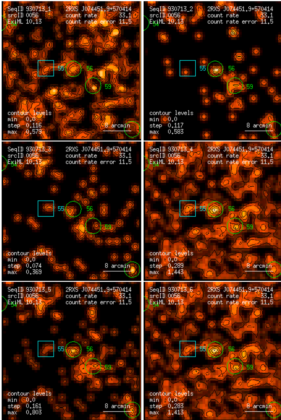
Figure 56: RASS 930713: detection 0056: band rate images, Gaussian filter: (1) PSPC channels 11 – 41, (2) 52 – 90, (3) 91 – 201, (4) 11 – 235, (5) 52 – 201, (6) 11 – 201. Broad band rates in counts/ks. Band rate contour levels in counts/ks/arcmin 2 .
