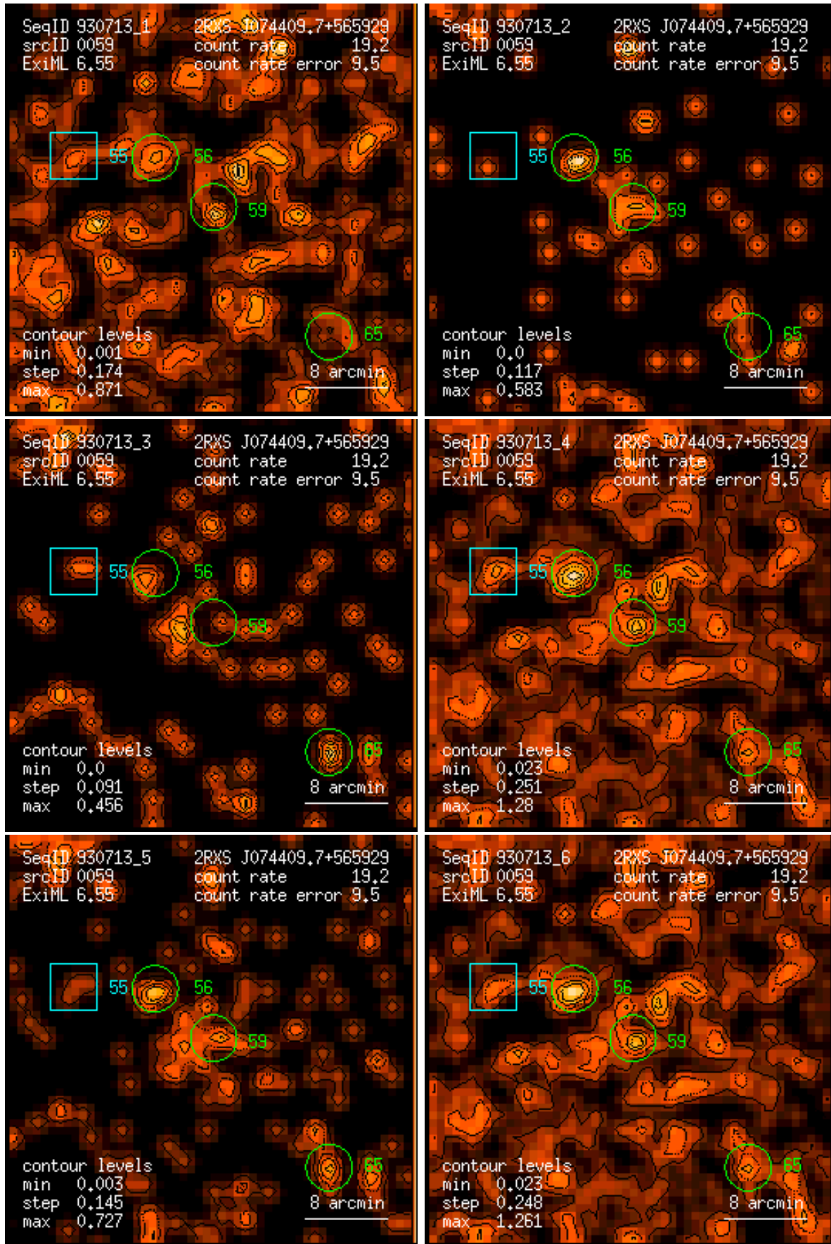
Figure 59: RASS 930713: detection 0059: band rate images, Gaussian filter: (1) PSPC channels 11 – 41, (2) 52 – 90, (3) 91 – 201, (4) 11 – 235, (5) 52 – 201, (6) 11 – 201. Broad band rates in counts/ks. Band rate contour levels in counts/ks/arcmin 2 .
