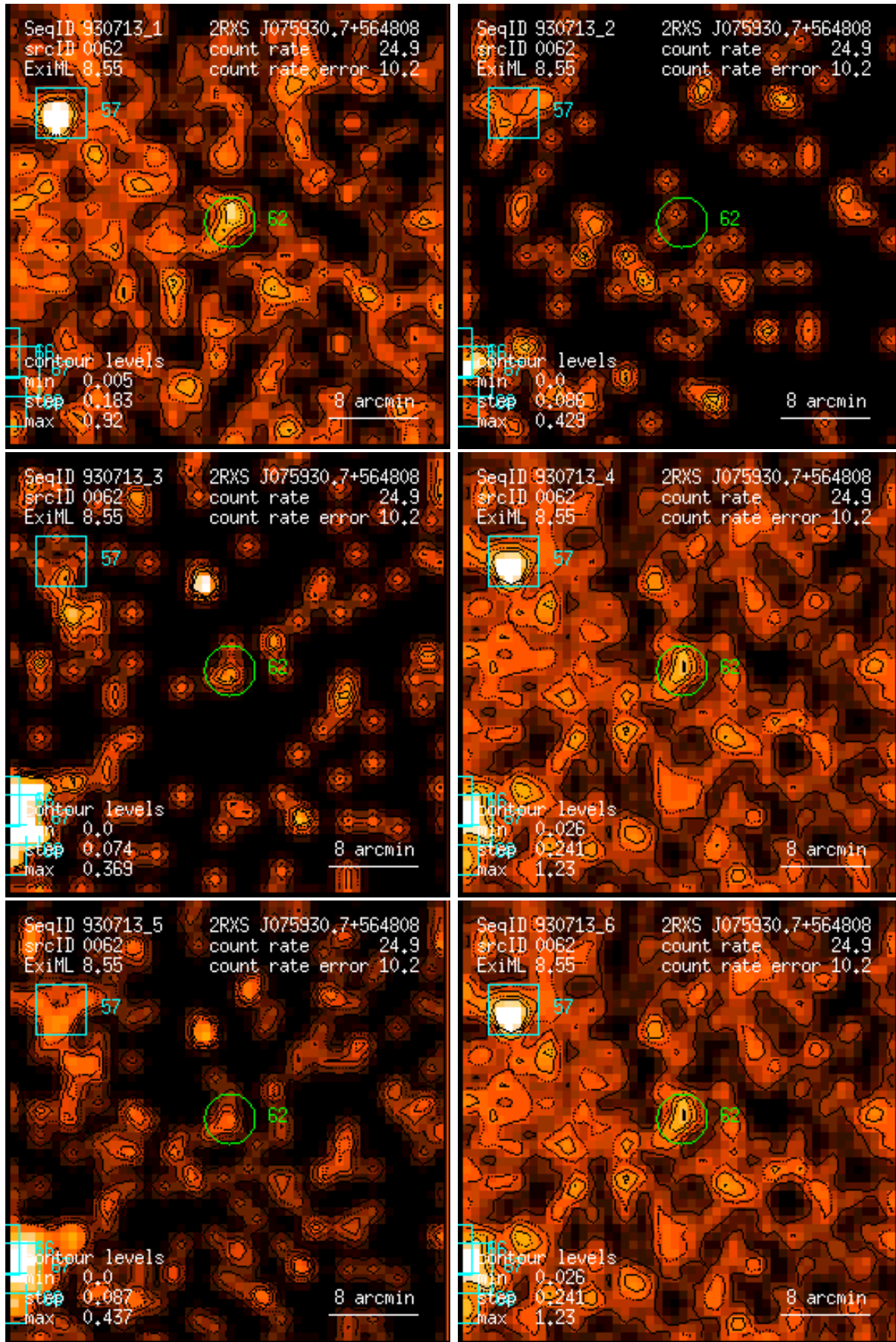
Figure 62: RASS 930713: detection 0062: band rate images, Gaussian filter: (1) PSPC channels 11 – 41, (2) 52 – 90, (3) 91 – 201, (4) 11 – 235, (5) 52 – 201, (6) 11 – 201. Broad band rates in counts/ks. Band rate contour levels in counts/ks/arcmin 2 .
