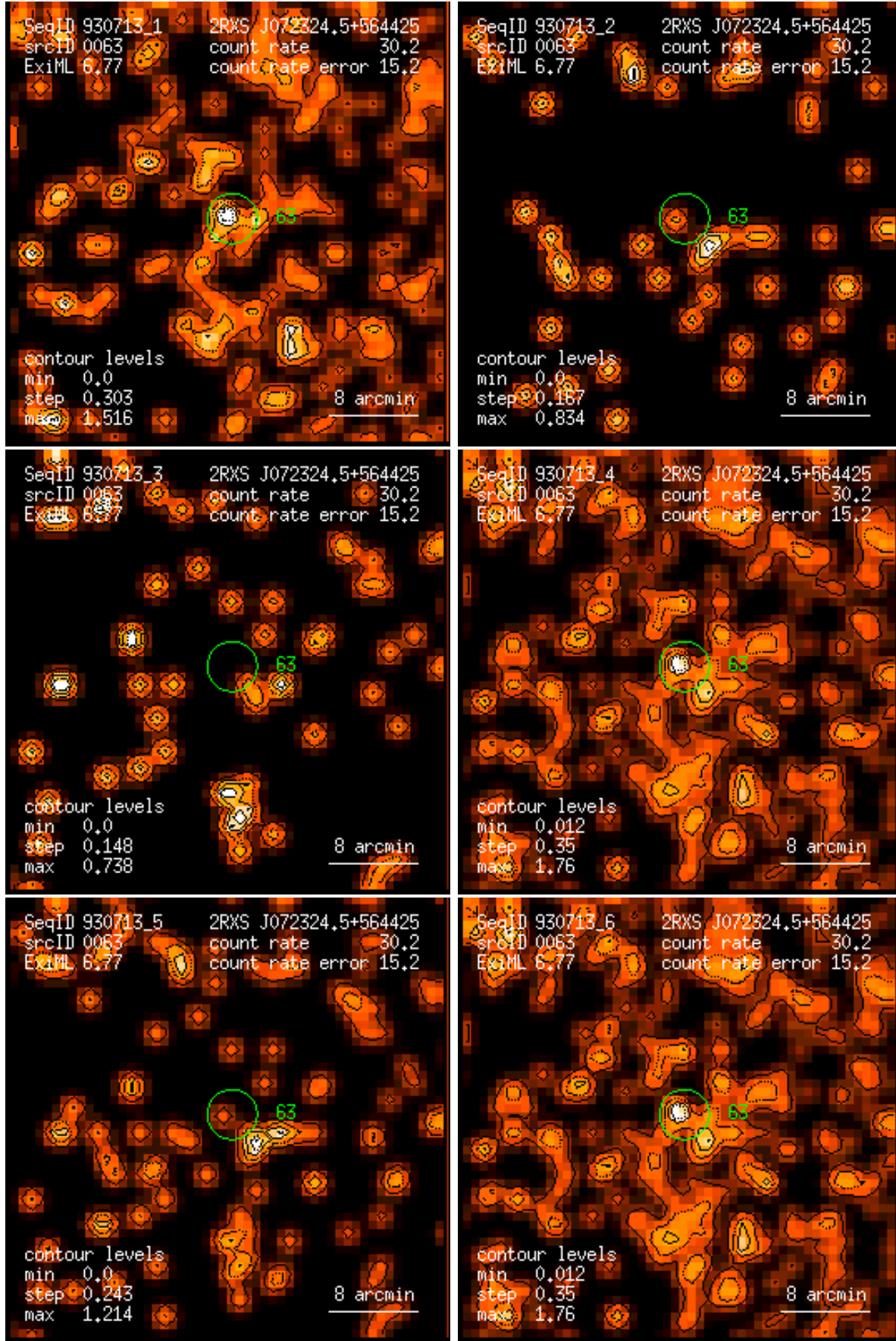
Figure 63: RASS 930713: detection 0063: band rate images, Gaussian filter: (1) PSPC channels 11 – 41, (2) 52 – 90, (3) 91 – 201, (4) 11 – 235, (5) 52 – 201, (6) 11 – 201. Broad band rates in counts/ks. Band rate contour levels in counts/ks/arcmin 2 .
