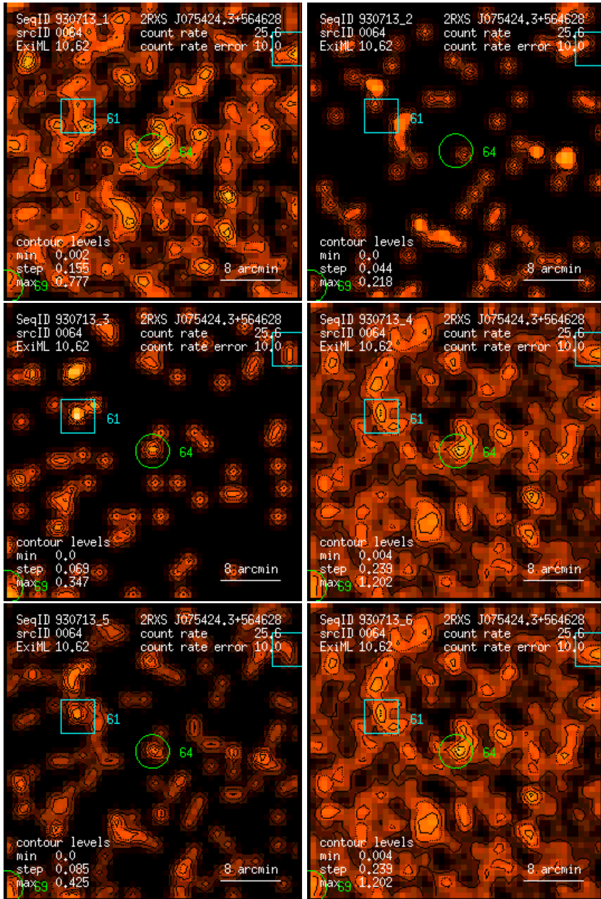
Figure 64: RASS 930713: detection 0064: band rate images, Gaussian filter: (1) PSPC channels 11 – 41, (2) 52 – 90, (3) 91 – 201, (4) 11 – 235, (5) 52 – 201, (6) 11 – 201. Broad band rates in counts/ks. Band rate contour levels in counts/ks/arcmin 2 .
