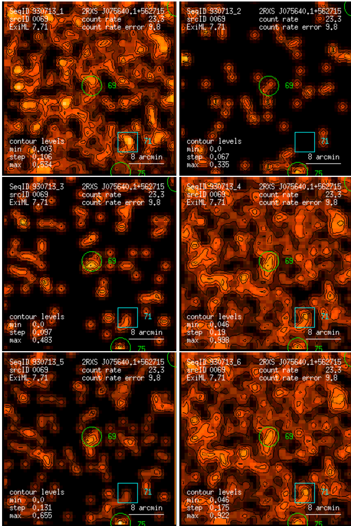
Figure 69: RASS 930713: detection 0069: band rate images, Gaussian filter: (1) PSPC channels 11 – 41, (2) 52 – 90, (3) 91 – 201, (4) 11 – 235, (5) 52 – 201, (6) 11 – 201. Broad band rates in counts/ks. Band rate contour levels in counts/ks/arcmin 2 .
