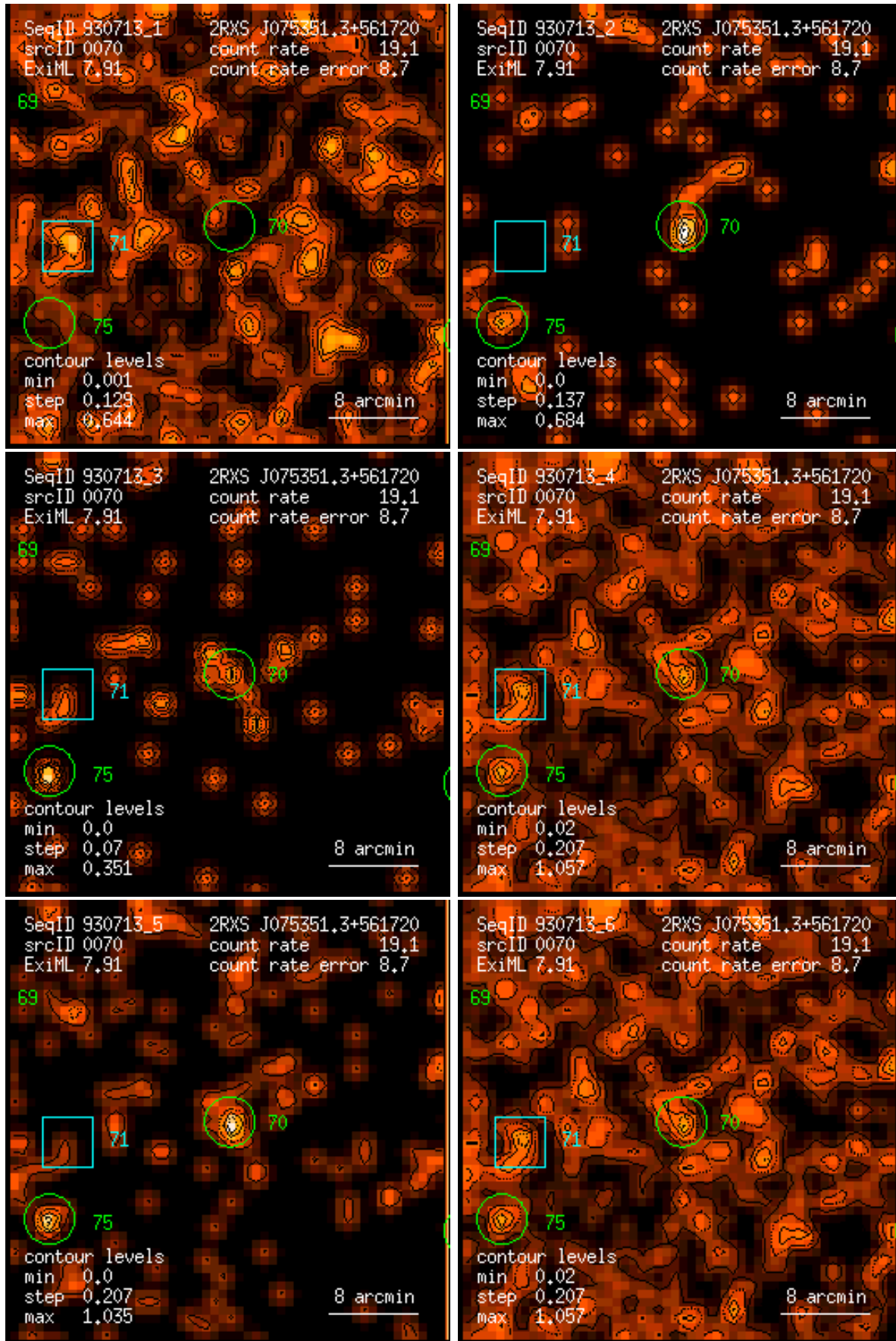
Figure 70: RASS 930713: detection 0070: band rate images, Gaussian filter: (1) PSPC channels 11 – 41, (2) 52 – 90, (3) 91 – 201, (4) 11 – 235, (5) 52 – 201, (6) 11 – 201. Broad band rates in counts/ks. Band rate contour levels in counts/ks/arcmin 2 .
