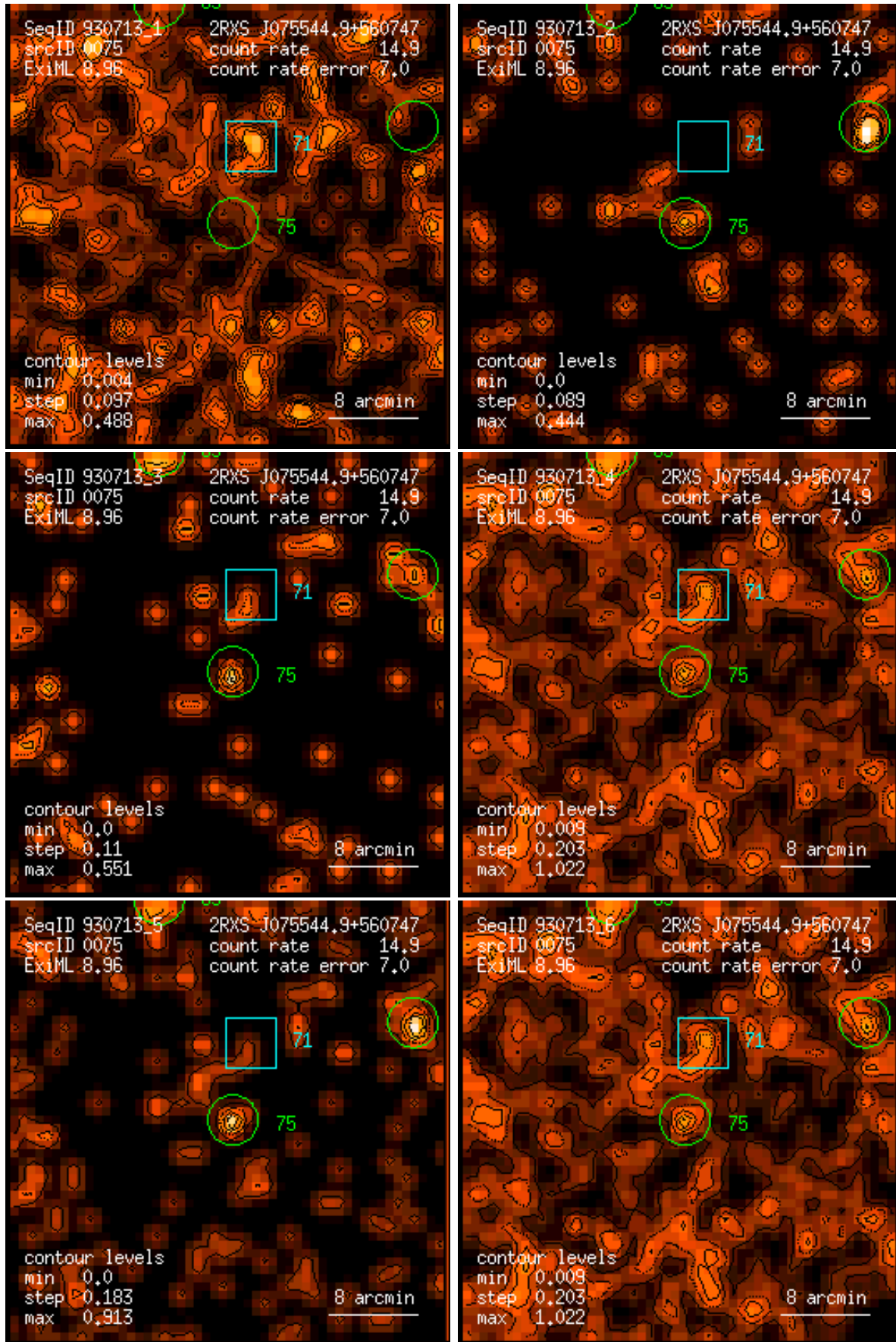
Figure 75: RASS 930713: detection 0075: band rate images, Gaussian filter: (1) PSPC channels 11 – 41, (2) 52 – 90, (3) 91 – 201, (4) 11 – 235, (5) 52 – 201, (6) 11 – 201. Broad band rates in counts/ks. Band rate contour levels in counts/ks/arcmin 2 .
