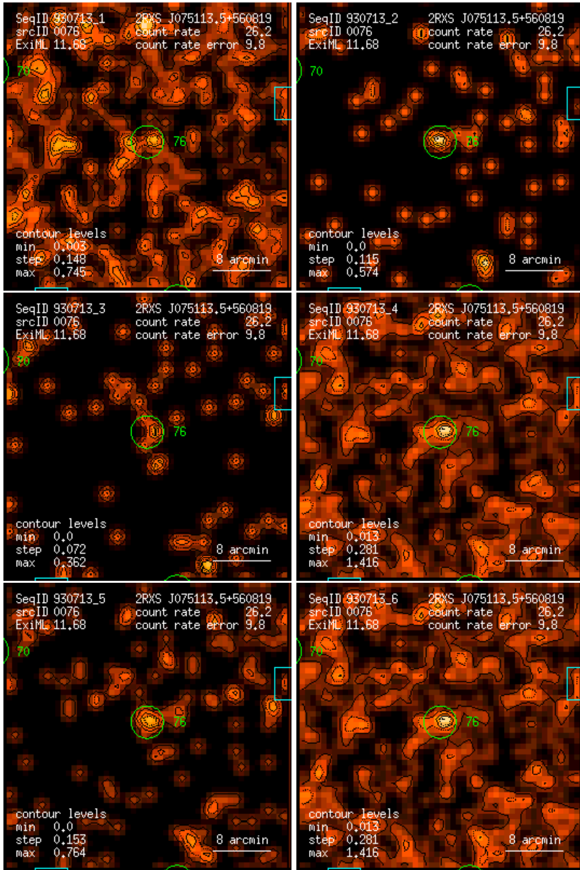
Figure 76: RASS 930713: detection 0076: band rate images, Gaussian filter: (1) PSPC channels 11 – 41, (2) 52 – 90, (3) 91 – 201, (4) 11 – 235, (5) 52 – 201, (6) 11 – 201. Broad band rates in counts/ks. Band rate contour levels in counts/ks/arcmin 2 .
