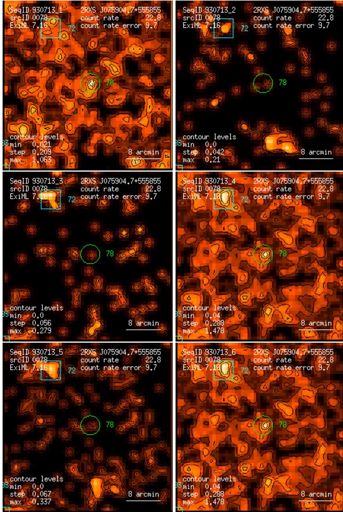
Figure 78: RASS 930713: detection 0078: band rate images, Gaussian filter: (1) PSPC channels 11 – 41, (2) 52 – 90, (3) 91 – 201, (4) 11 – 235, (5) 52 – 201, (6) 11 – 201. Broad band rates in counts/ks. Band rate contour levels in counts/ks/arcmin 2 .
