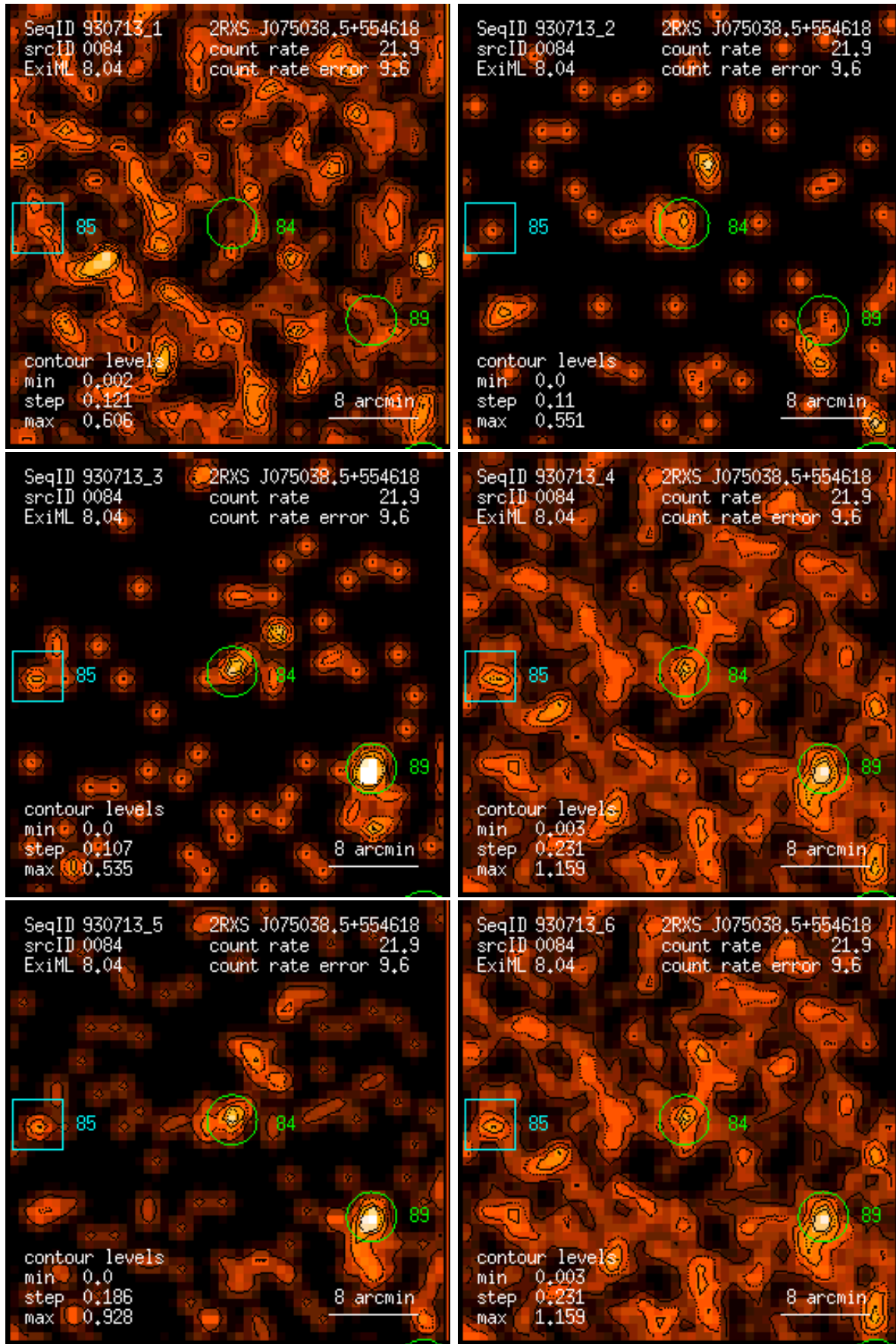
Figure 84: RASS 930713: detection 0084: band rate images, Gaussian filter: (1) PSPC channels 11 – 41, (2) 52 – 90, (3) 91 – 201, (4) 11 – 235, (5) 52 – 201, (6) 11 – 201. Broad band rates in counts/ks. Band rate contour levels in counts/ks/arcmin 2 .
