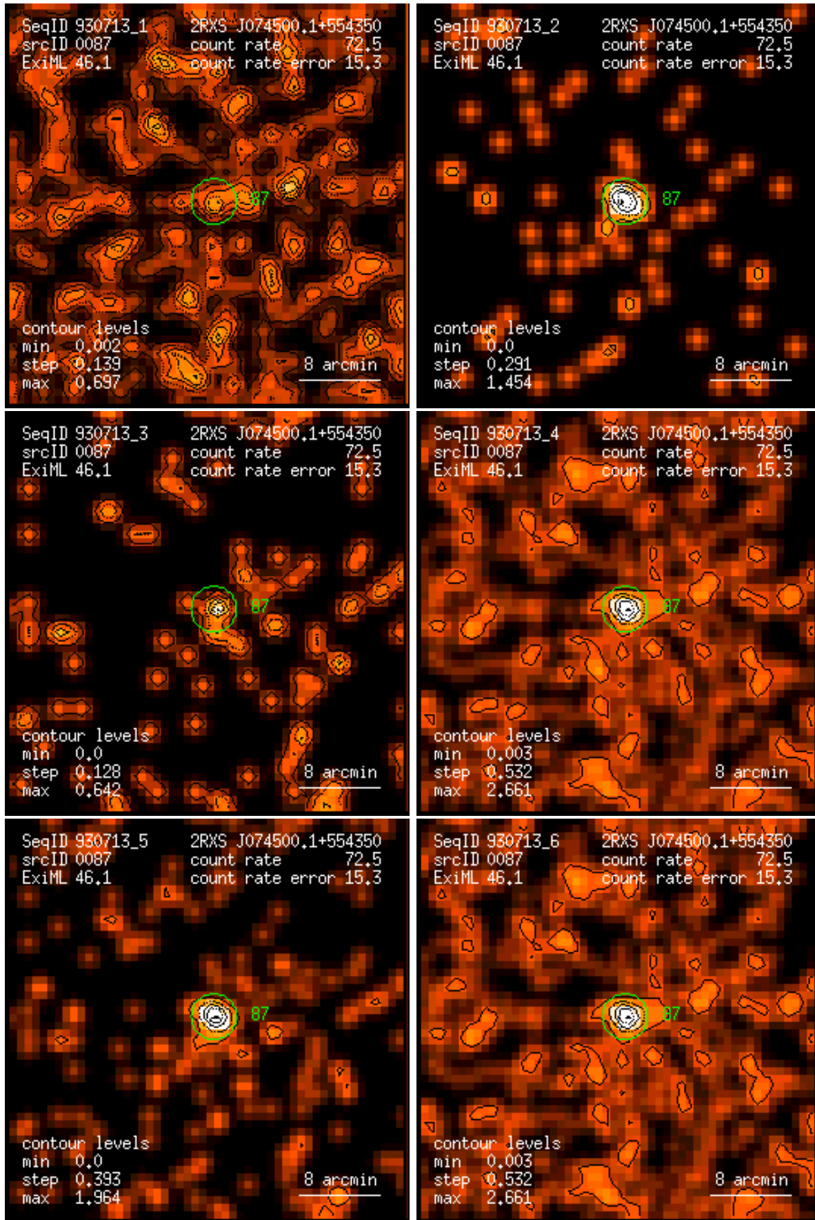
Figure 87: RASS 930713: detection 0087: band rate images, Gaussian filter: (1) PSPC channels 11 – 41, (2) 52 – 90, (3) 91 – 201, (4) 11 – 235, (5) 52 – 201, (6) 11 – 201. Broad band rates in counts/ks. Band rate contour levels in counts/ks/arcmin 2 .
