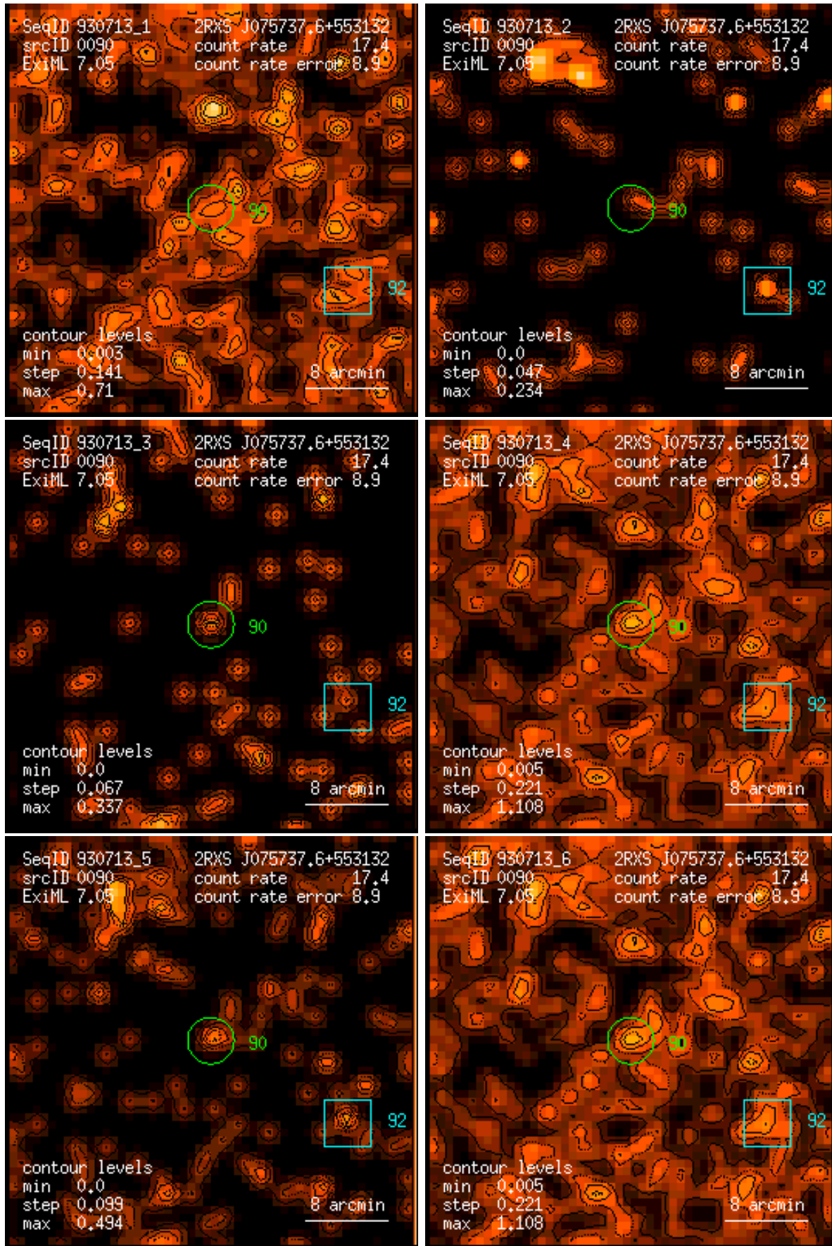
Figure 90: RASS 930713: detection 0090: band rate images, Gaussian filter: (1) PSPC channels 11 – 41, (2) 52 – 90, (3) 91 – 201, (4) 11 – 235, (5) 52 – 201, (6) 11 – 201. Broad band rates in counts/ks. Band rate contour levels in counts/ks/arcmin 2 .
