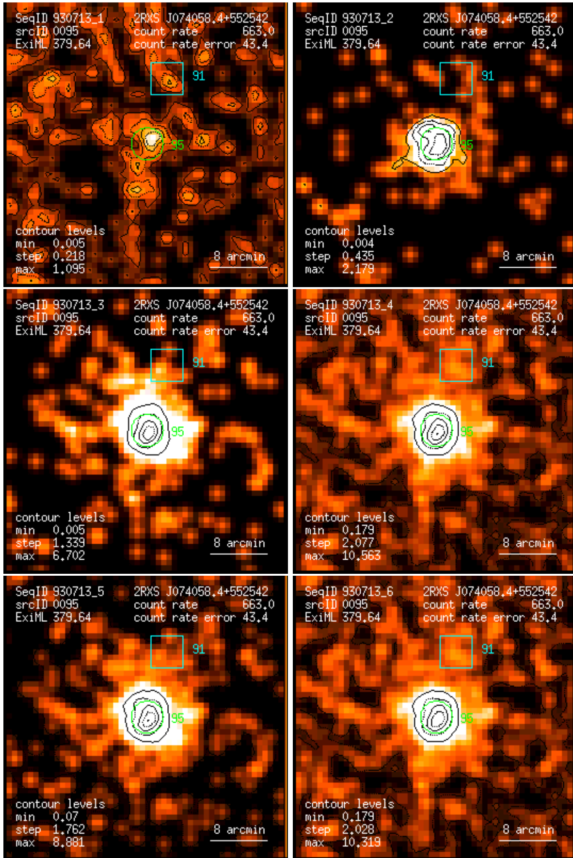
Figure 95: RASS 930713: detection 0095: band rate images, Gaussian filter: (1) PSPC channels 11 – 41, (2) 52 – 90, (3) 91 – 201, (4) 11 – 235, (5) 52 – 201, (6) 11 – 201. Broad band rates in counts/ks. Band rate contour levels in counts/ks/arcmin 2 .
