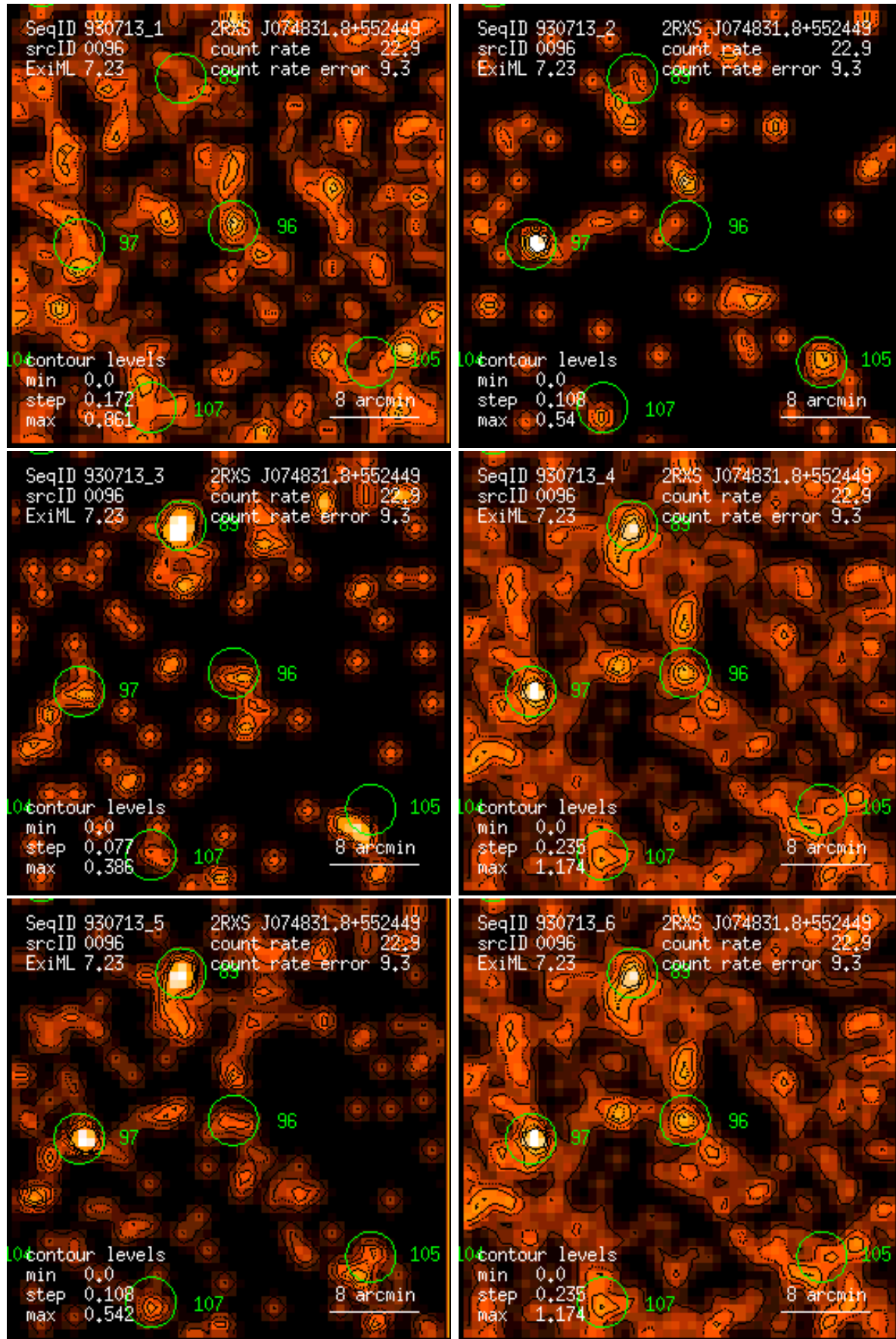
Figure 96: RASS 930713: detection 0096: band rate images, Gaussian filter: (1) PSPC channels 11 – 41, (2) 52 – 90, (3) 91 – 201, (4) 11 – 235, (5) 52 – 201, (6) 11 – 201. Broad band rates in counts/ks. Band rate contour levels in counts/ks/arcmin 2 .
