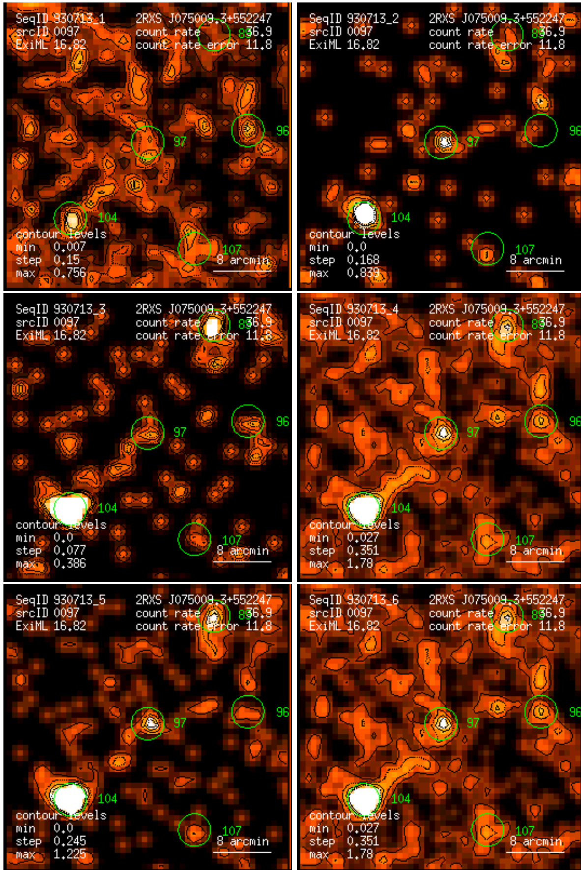
Figure 97: RASS 930713: detection 0097: band rate images, Gaussian filter: (1) PSPC channels 11 – 41, (2) 52 – 90, (3) 91 – 201, (4) 11 – 235, (5) 52 – 201, (6) 11 – 201. Broad band rates in counts/ks. Band rate contour levels in counts/ks/arcmin 2 .
