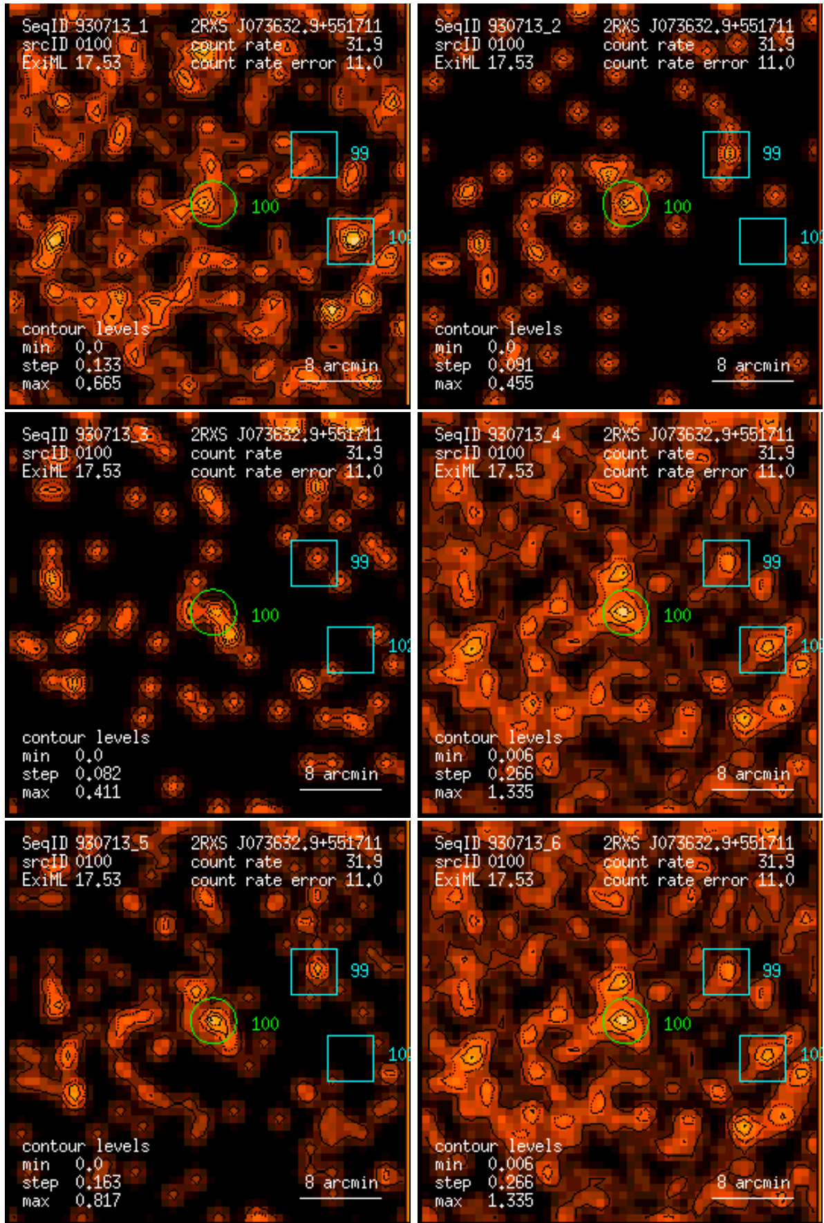
Figure 100: RASS 930713: detection 0100: band rate images, Gaussian filter: (1) PSPC channels 11 – 41, (2) 52 – 90, (3) 91 – 201, (4) 11 – 235, (5) 52 – 201, (6) 11 – 201. Broad band rates in counts/ks. Band rate contour levels in counts/ks/arcmin 2 .
