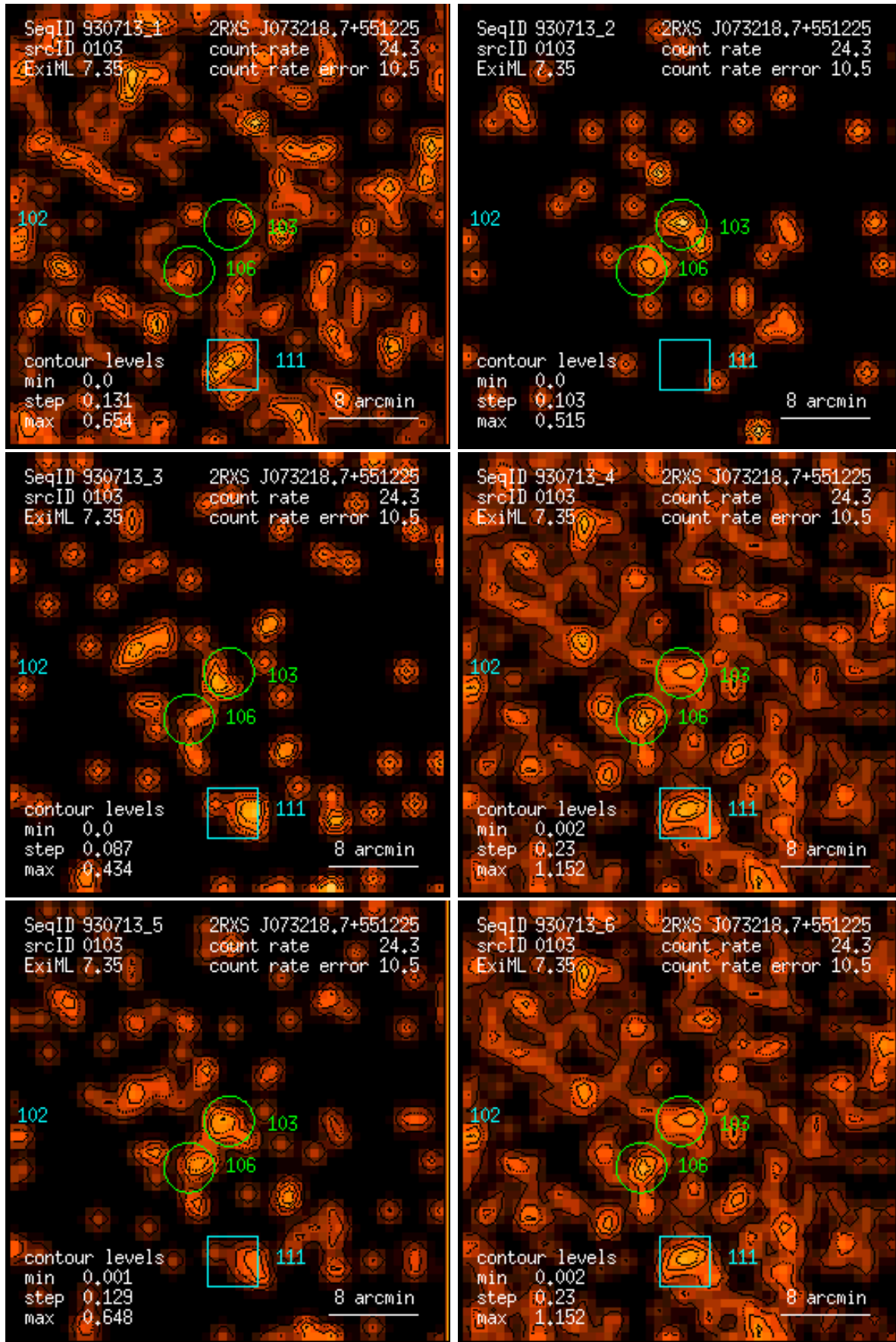
Figure 103: RASS 930713: detection 0103: band rate images, Gaussian filter: (1) PSPC channels 11 – 41, (2) 52 – 90, (3) 91 – 201, (4) 11 – 235, (5) 52 – 201, (6) 11 – 201. Broad band rates in counts/ks. Band rate contour levels in counts/ks/arcmin 2 .
