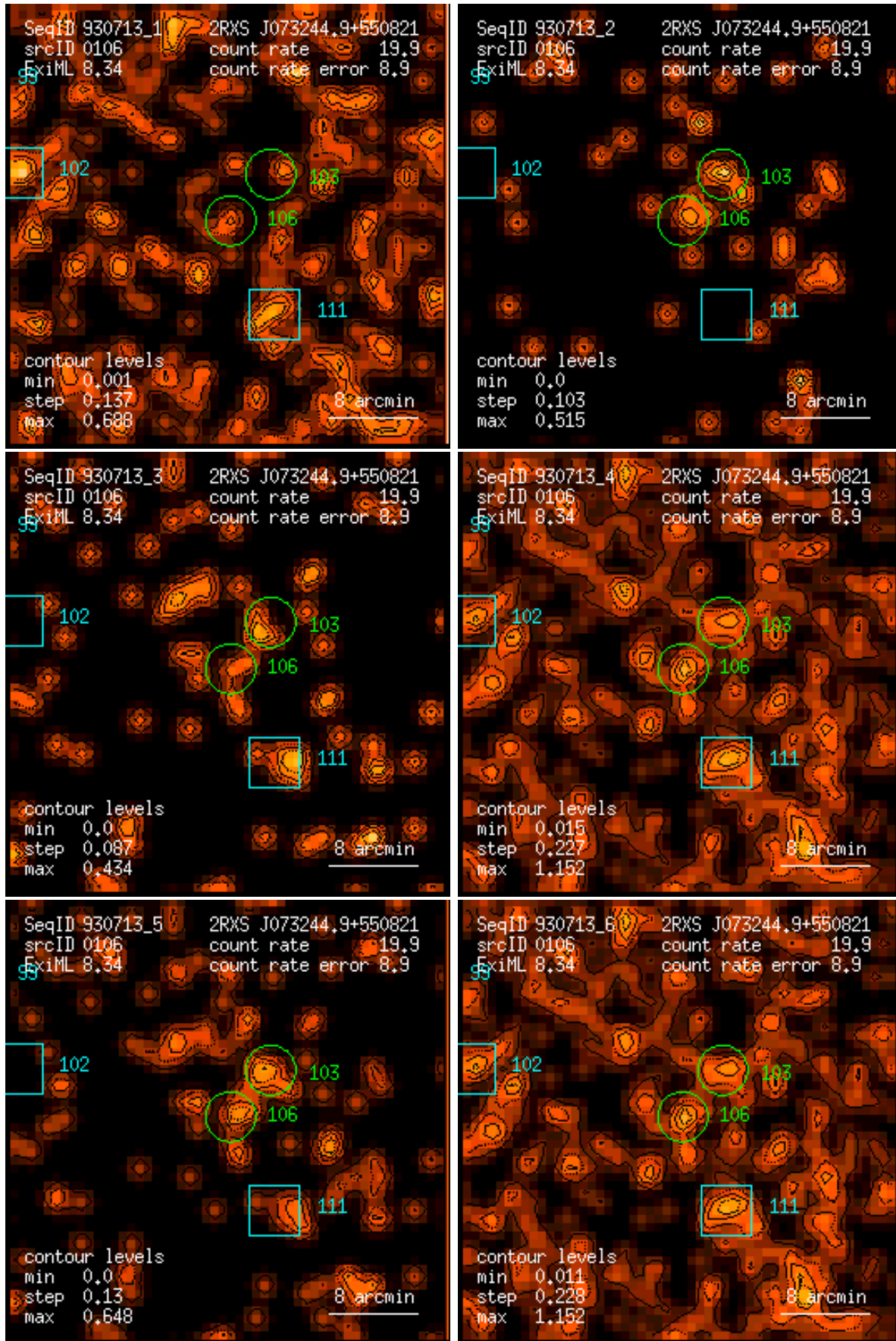
Figure 106: RASS 930713: detection 0106: band rate images, Gaussian filter: (1) PSPC channels 11 – 41, (2) 52 – 90, (3) 91 – 201, (4) 11 – 235, (5) 52 – 201, (6) 11 – 201. Broad band rates in counts/ks. Band rate contour levels in counts/ks/arcmin 2 .
